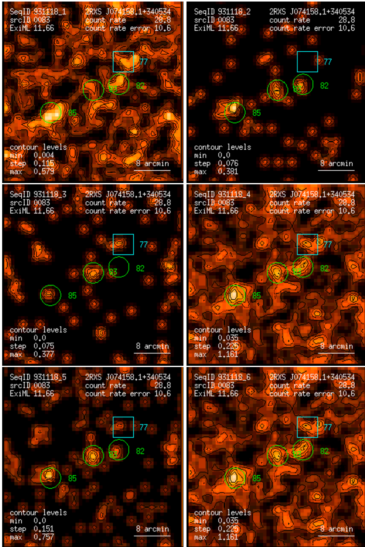
Figure 83: RASS 931118: detection 0083: band rate images, Gaussian filter: (1) PSPC channels 11 – 41, (2) 52 – 90, (3) 91 – 201, (4) 11 – 235, (5) 52 – 201, (6) 11 – 201. Broad band rates in counts/ks. Band rate contour levels in counts/ks/arcmin 2 .
