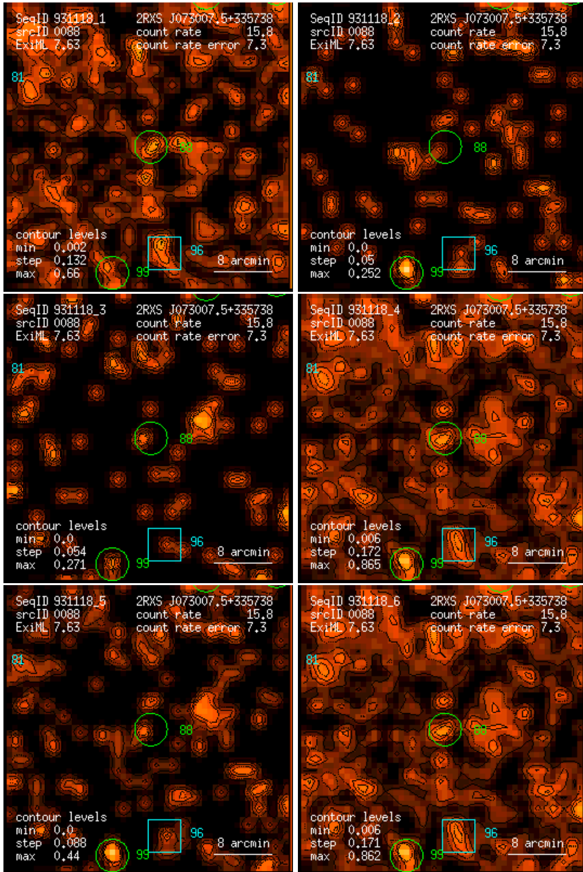
Figure 88: RASS 931118: detection 0088: band rate images, Gaussian filter: (1) PSPC channels 11 – 41, (2) 52 – 90, (3) 91 – 201, (4) 11 – 235, (5) 52 – 201, (6) 11 – 201. Broad band rates in counts/ks. Band rate contour levels in counts/ks/arcmin 2 .
