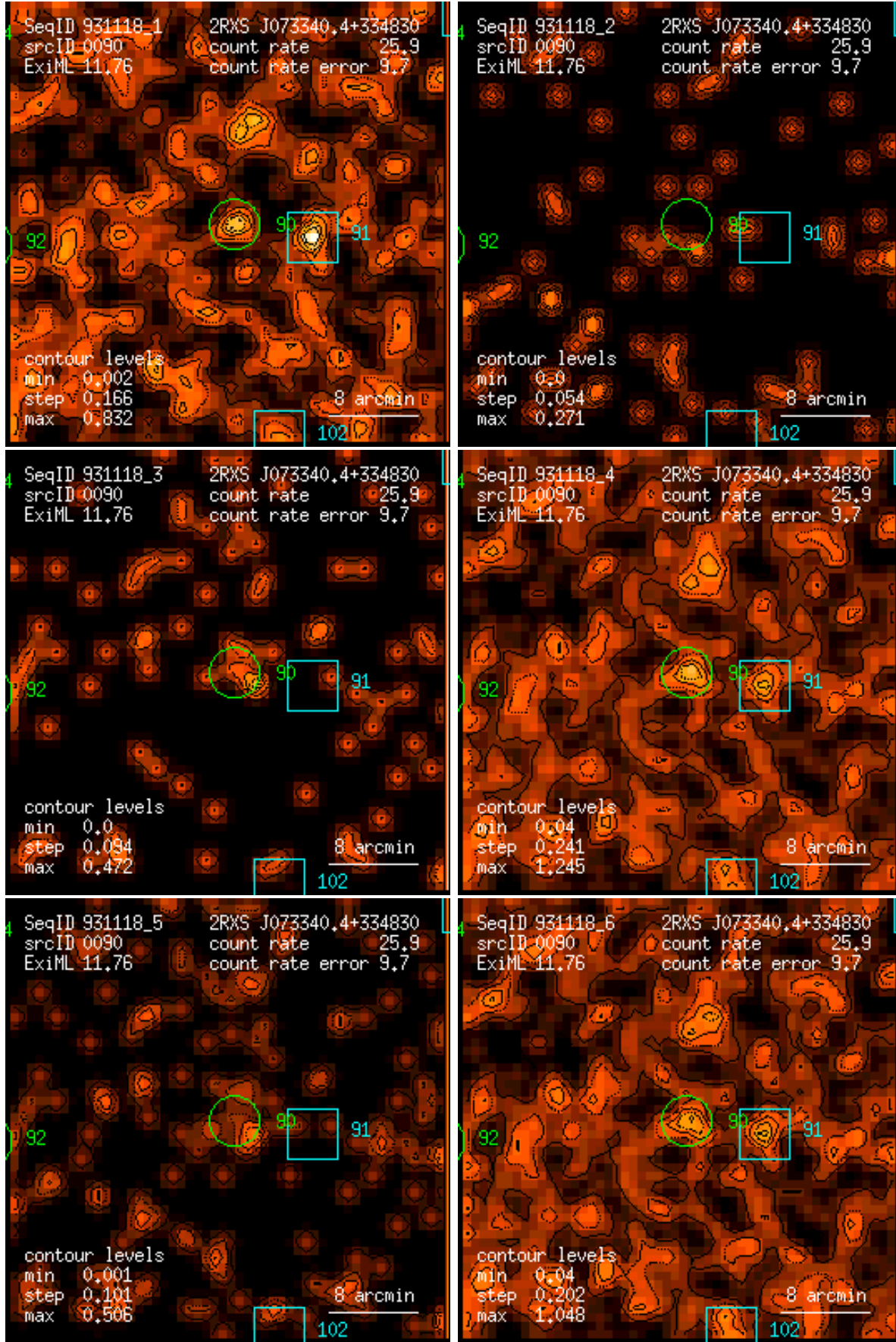
Figure 90: RASS 931118: detection 0090: band rate images, Gaussian filter: (1) PSPC channels 11 – 41, (2) 52 – 90, (3) 91 – 201, (4) 11 – 235, (5) 52 – 201, (6) 11 – 201. Broad band rates in counts/ks. Band rate contour levels in counts/ks/arcmin 2 .
