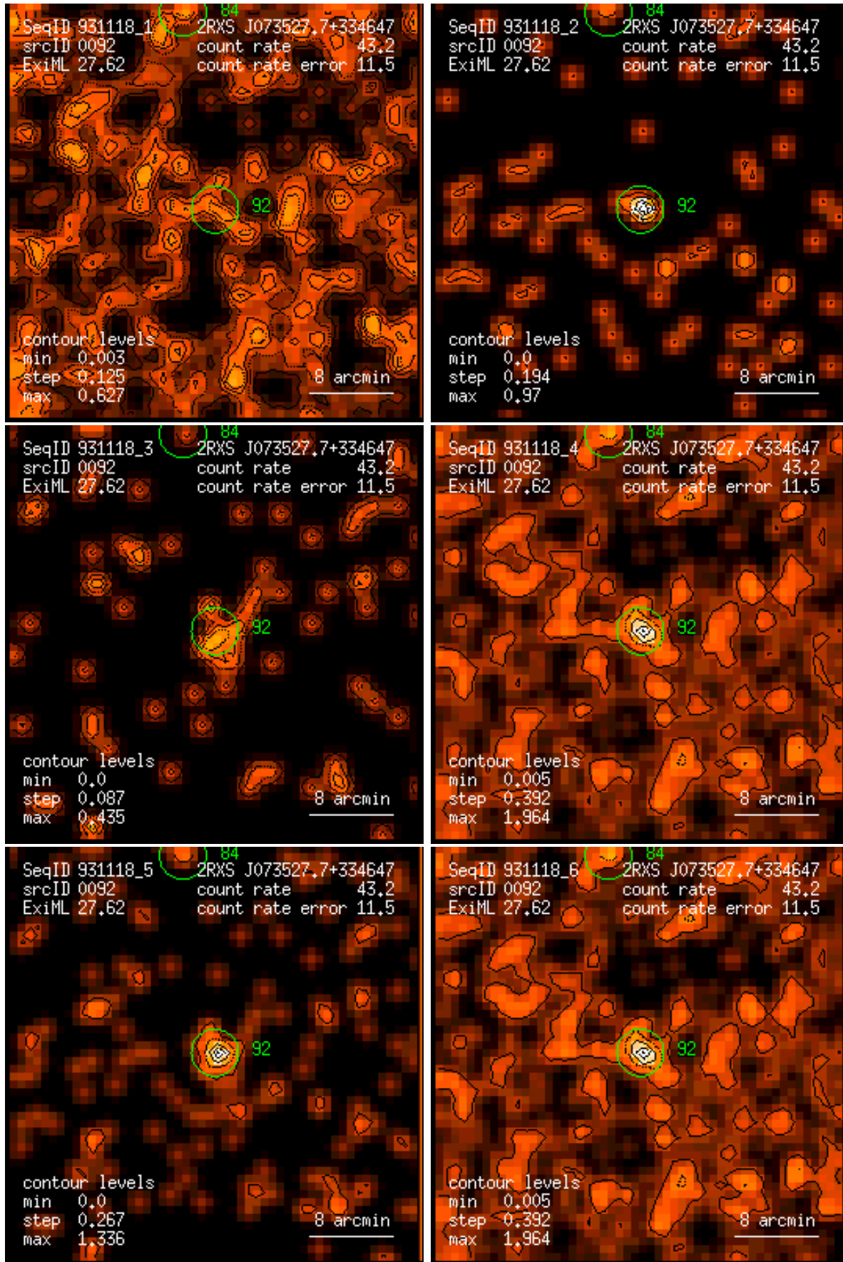
Figure 92: RASS 931118: detection 0092: band rate images, Gaussian filter: (1) PSPC channels 11 – 41, (2) 52 – 90, (3) 91 – 201, (4) 11 – 235, (5) 52 – 201, (6) 11 – 201. Broad band rates in counts/ks. Band rate contour levels in counts/ks/arcmin 2 .
