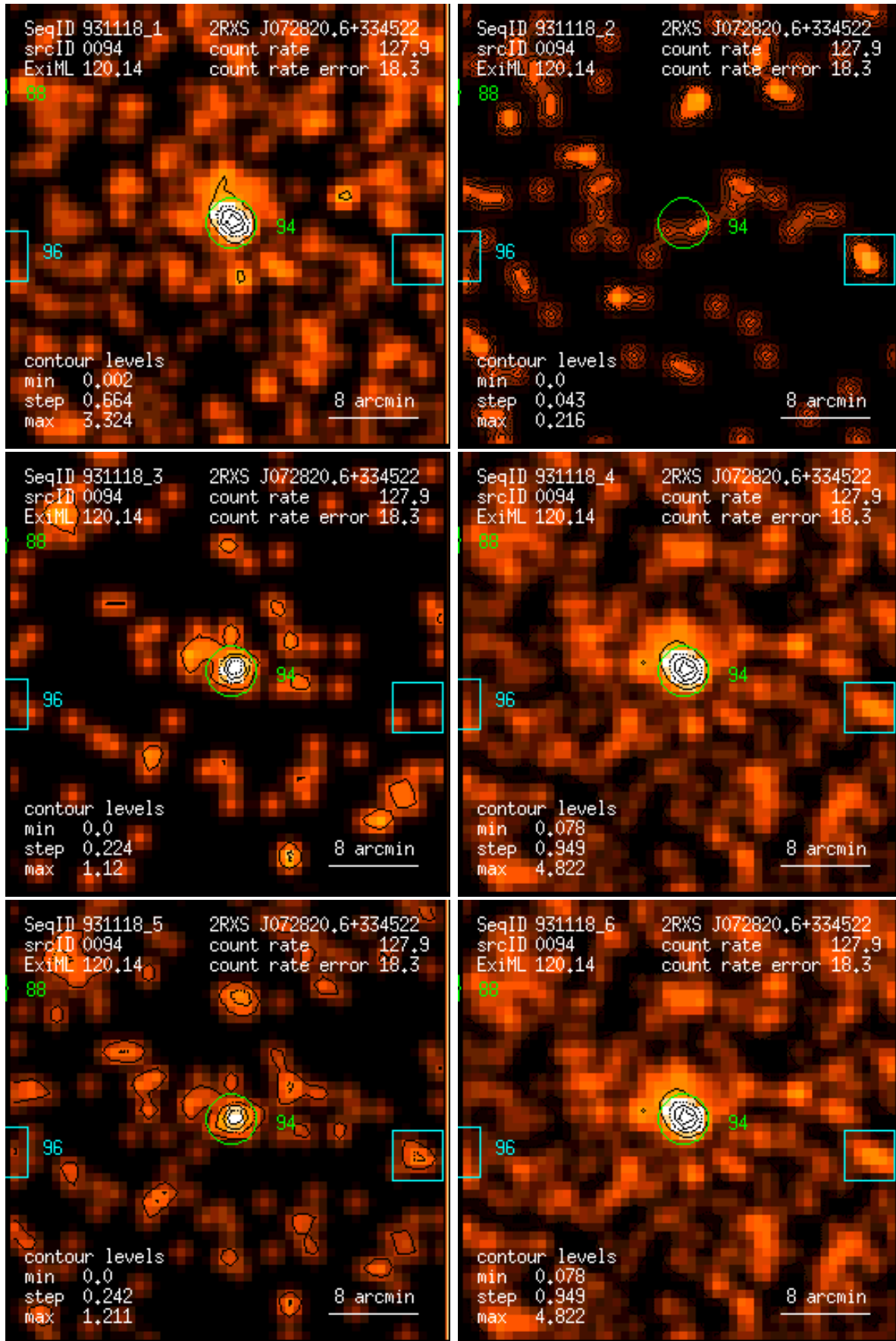
Figure 94: RASS 931118: detection 0094: band rate images, Gaussian filter: (1) PSPC channels 11 – 41, (2) 52 – 90, (3) 91 – 201, (4) 11 – 235, (5) 52 – 201, (6) 11 – 201. Broad band rates in counts/ks. Band rate contour levels in counts/ks/arcmin 2 .
