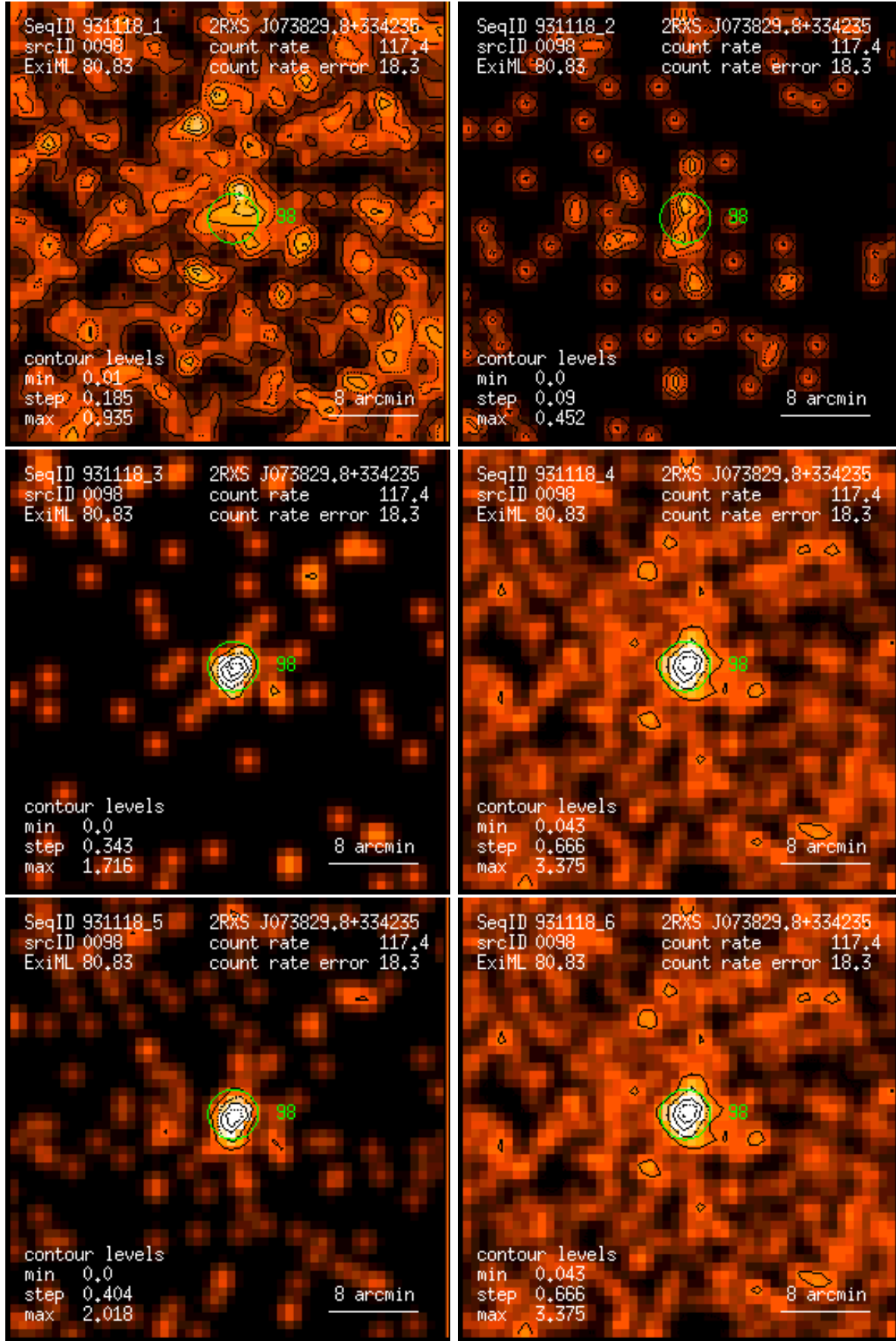
Figure 98: RASS 931118: detection 0098: band rate images, Gaussian filter: (1) PSPC channels 11 – 41, (2) 52 – 90, (3) 91 – 201, (4) 11 – 235, (5) 52 – 201, (6) 11 – 201. Broad band rates in counts/ks. Band rate contour levels in counts/ks/arcmin 2 .
