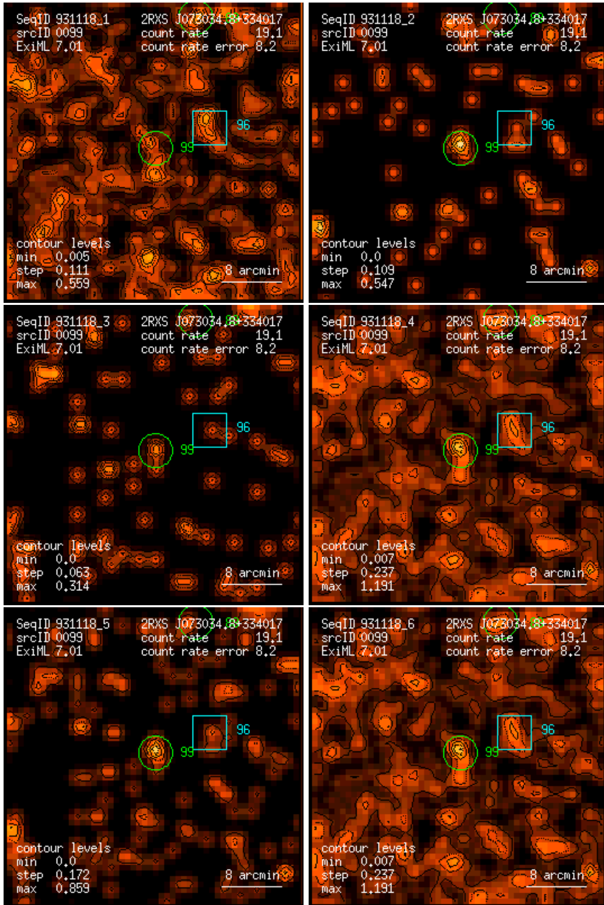
Figure 99: RASS 931118: detection 0099: band rate images, Gaussian filter: (1) PSPC channels 11 – 41, (2) 52 – 90, (3) 91 – 201, (4) 11 – 235, (5) 52 – 201, (6) 11 – 201. Broad band rates in counts/ks. Band rate contour levels in counts/ks/arcmin 2 .
