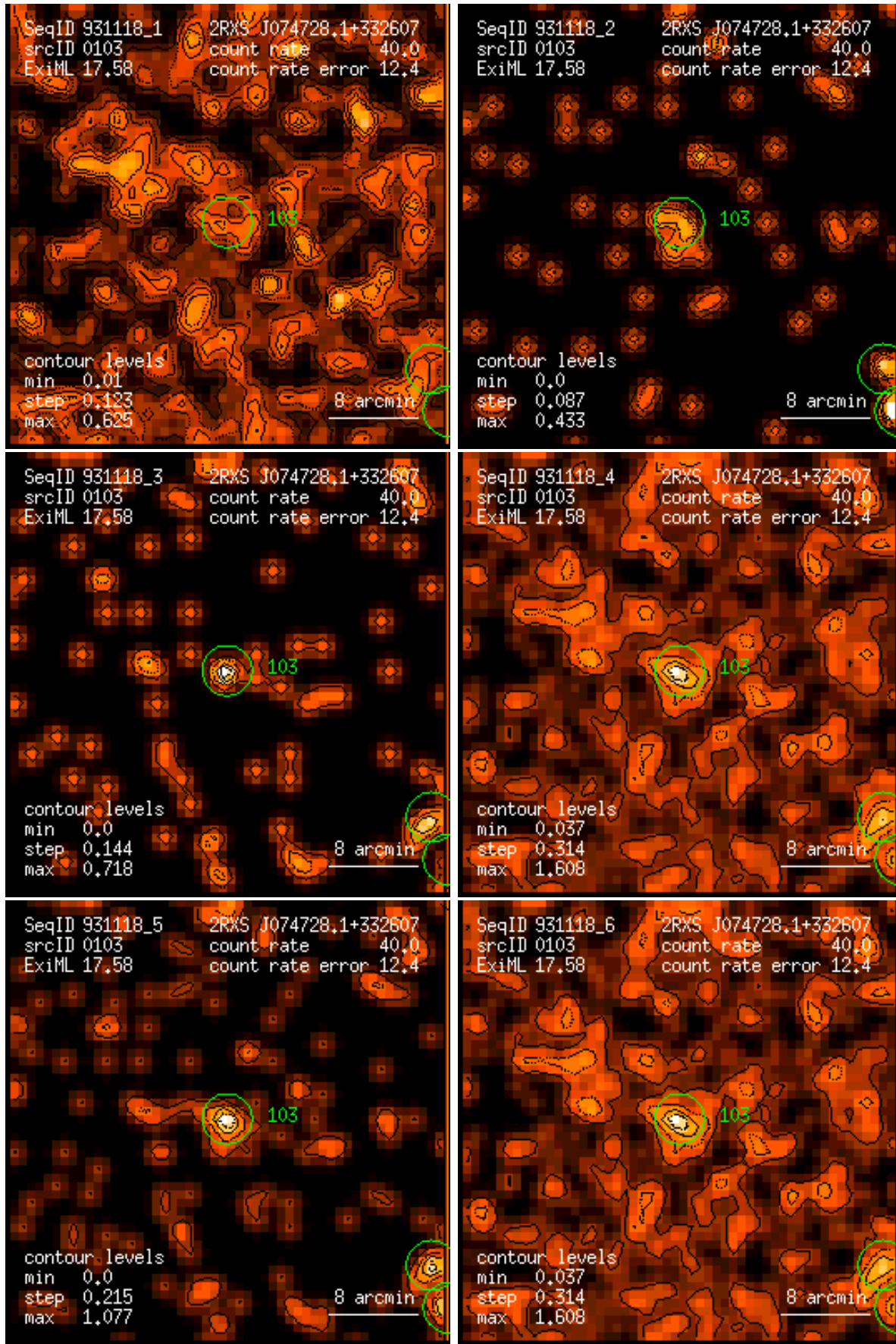
Figure 103: RASS 931118: detection 0103: band rate images, Gaussian filter: (1) PSPC channels 11 – 41, (2) 52 – 90, (3) 91 – 201, (4) 11 – 235, (5) 52 – 201, (6) 11 – 201. Broad band rates in counts/ks. Band rate contour levels in counts/ks/arcmin 2 .
