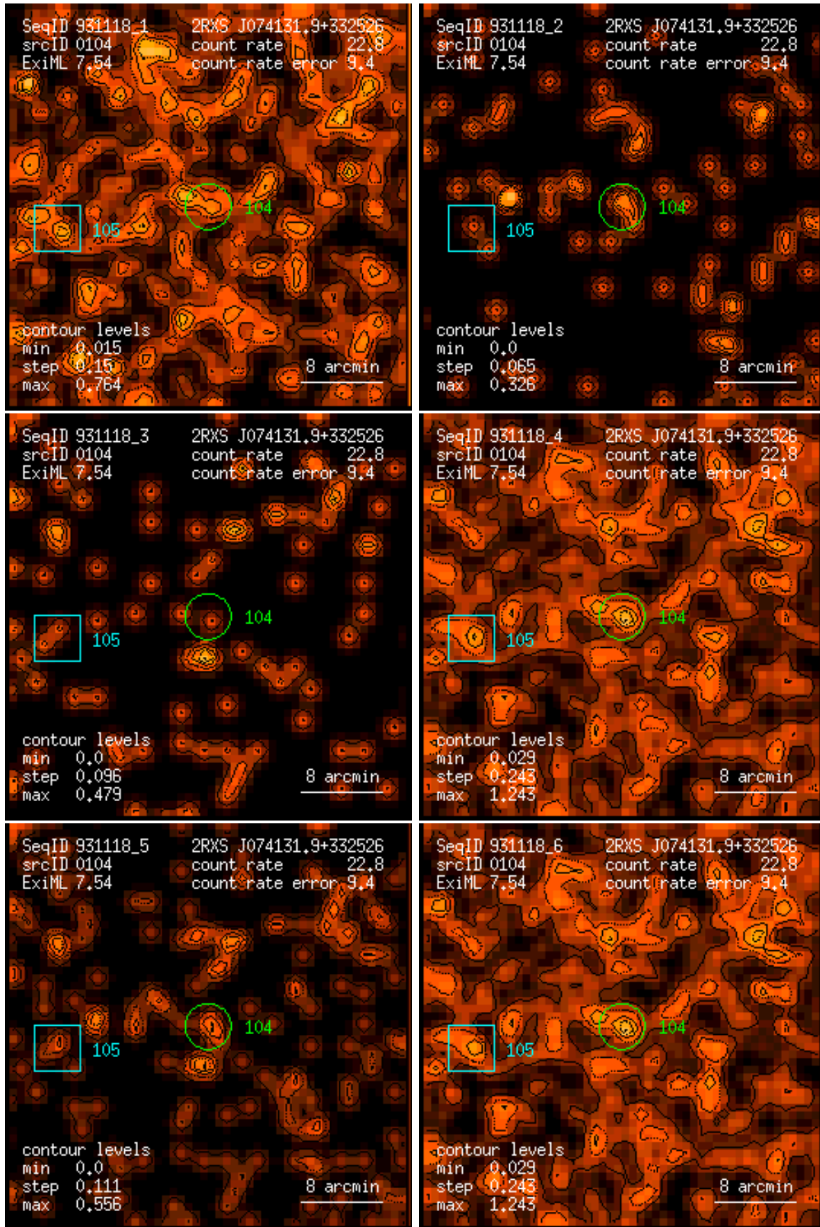
Figure 104: RASS 931118: detection 0104: band rate images, Gaussian filter: (1) PSPC channels 11 – 41, (2) 52 – 90, (3) 91 – 201, (4) 11 – 235, (5) 52 – 201, (6) 11 – 201. Broad band rates in counts/ks. Band rate contour levels in counts/ks/arcmin 2 .
