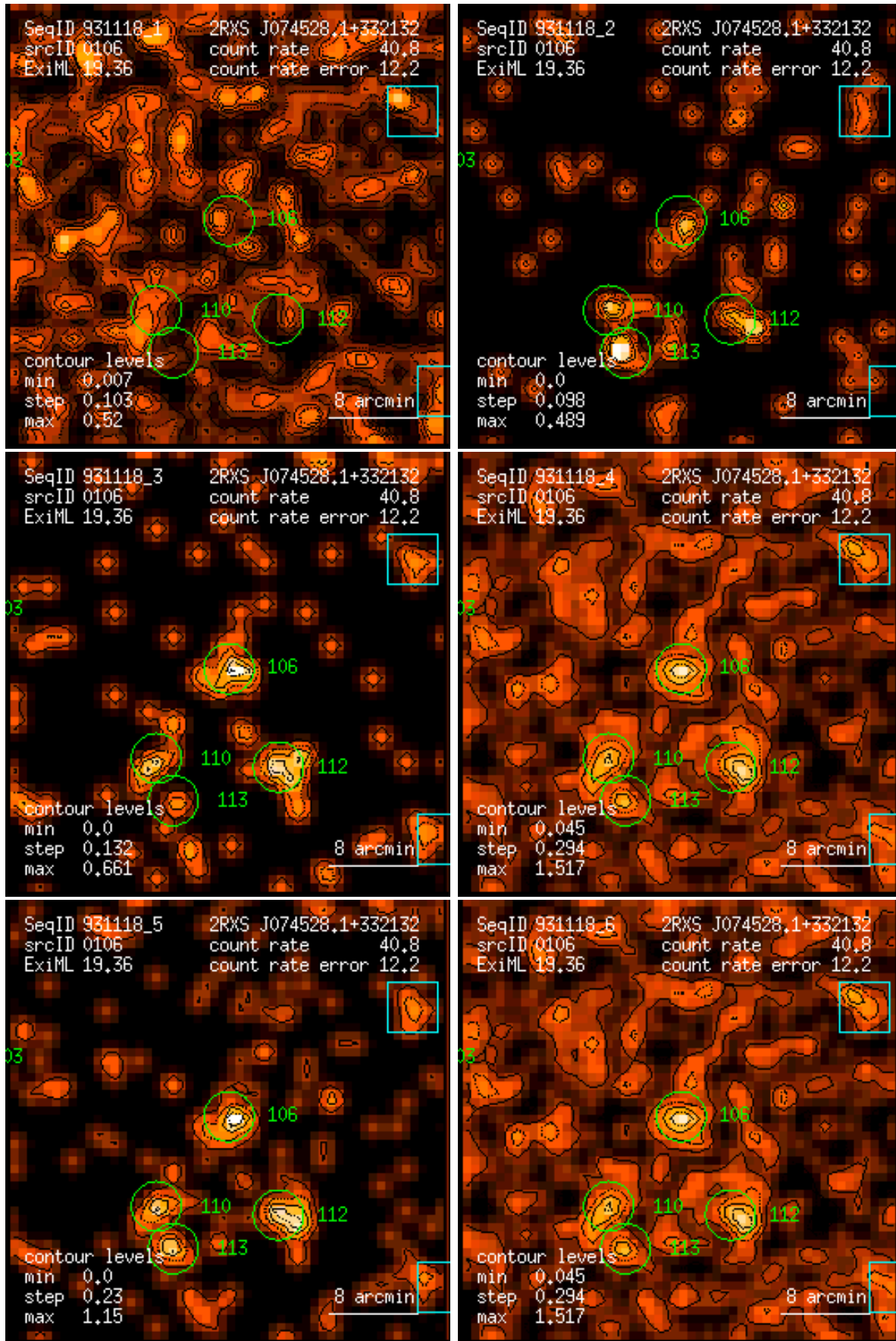
Figure 106: RASS 931118: detection 0106: band rate images, Gaussian filter: (1) PSPC channels 11 – 41, (2) 52 – 90, (3) 91 – 201, (4) 11 – 235, (5) 52 – 201, (6) 11 – 201. Broad band rates in counts/ks. Band rate contour levels in counts/ks/arcmin 2 .
