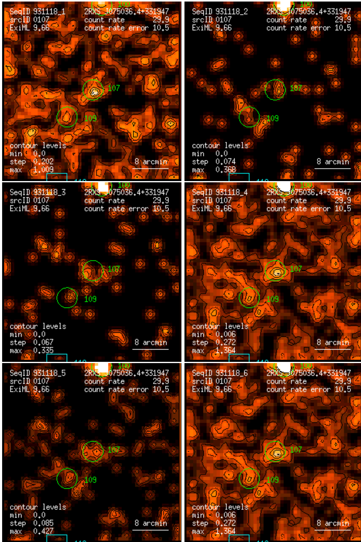
Figure 107: RASS 931118: detection 0107: band rate images, Gaussian filter: (1) PSPC channels 11 – 41, (2) 52 – 90, (3) 91 – 201, (4) 11 – 235, (5) 52 – 201, (6) 11 – 201. Broad band rates in counts/ks. Band rate contour levels in counts/ks/arcmin 2 .
