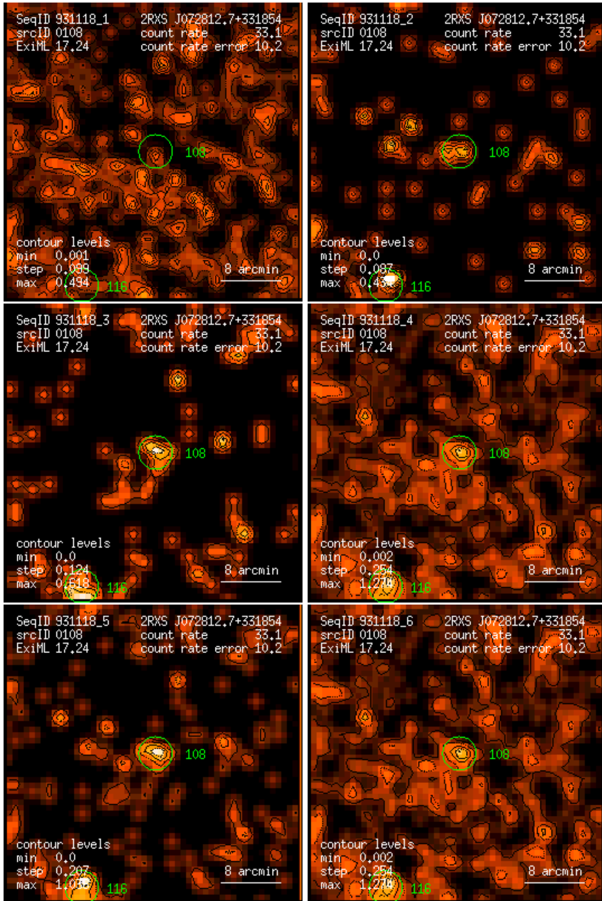
Figure 108: RASS 931118: detection 0108: band rate images, Gaussian filter: (1) PSPC channels 11 – 41, (2) 52 – 90, (3) 91 – 201, (4) 11 – 235, (5) 52 – 201, (6) 11 – 201. Broad band rates in counts/ks. Band rate contour levels in counts/ks/arcmin 2 .
