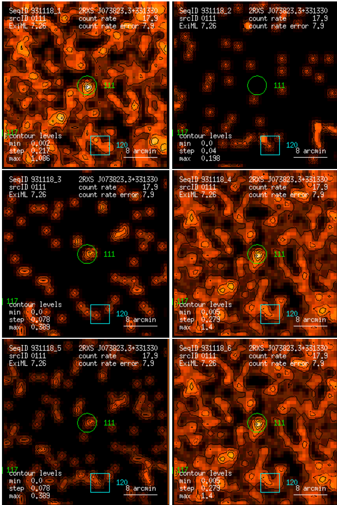
Figure 111: RASS 931118: detection 0111: band rate images, Gaussian filter: (1) PSPC channels 11 – 41, (2) 52 – 90, (3) 91 – 201, (4) 11 – 235, (5) 52 – 201, (6) 11 – 201. Broad band rates in counts/ks. Band rate contour levels in counts/ks/arcmin 2 .
