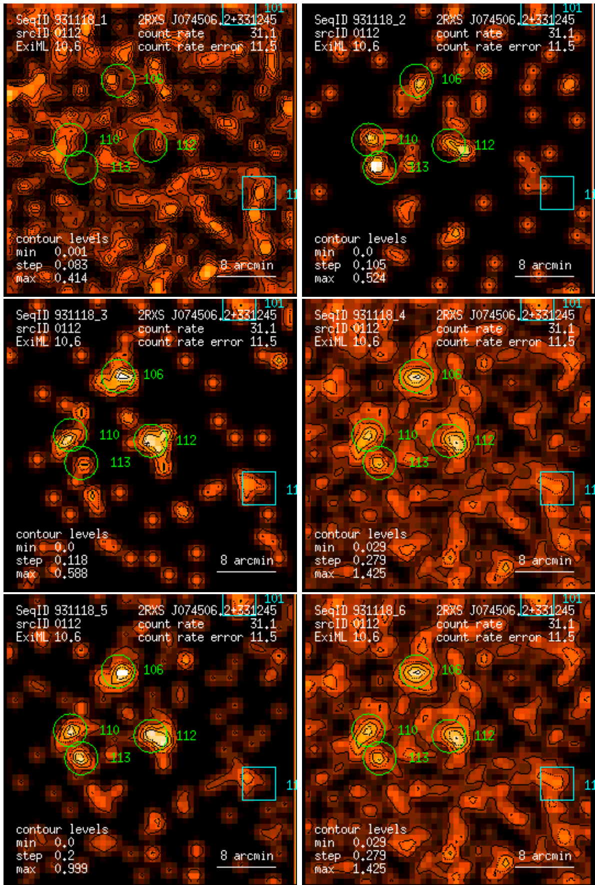
Figure 112: RASS 931118: detection 0112: band rate images, Gaussian filter: (1) PSPC channels 11 – 41, (2) 52 – 90, (3) 91 – 201, (4) 11 – 235, (5) 52 – 201, (6) 11 – 201. Broad band rates in counts/ks. Band rate contour levels in counts/ks/arcmin 2 .
