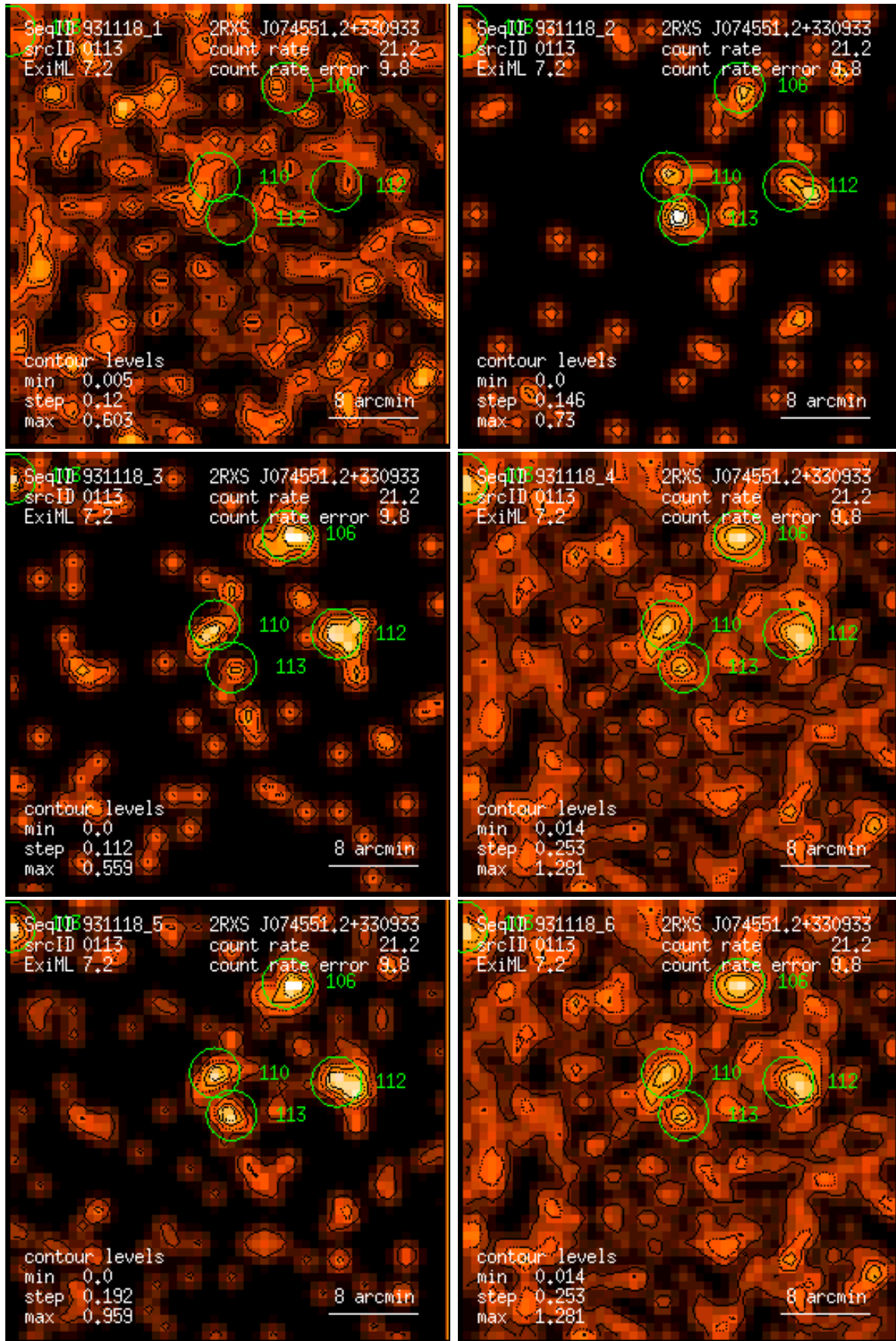
Figure 113: RASS 931118: detection 0113: band rate images, Gaussian filter: (1) PSPC channels 11 – 41, (2) 52 – 90, (3) 91 – 201, (4) 11 – 235, (5) 52 – 201, (6) 11 – 201. Broad band rates in counts/ks. Band rate contour levels in counts/ks/arcmin 2 .
