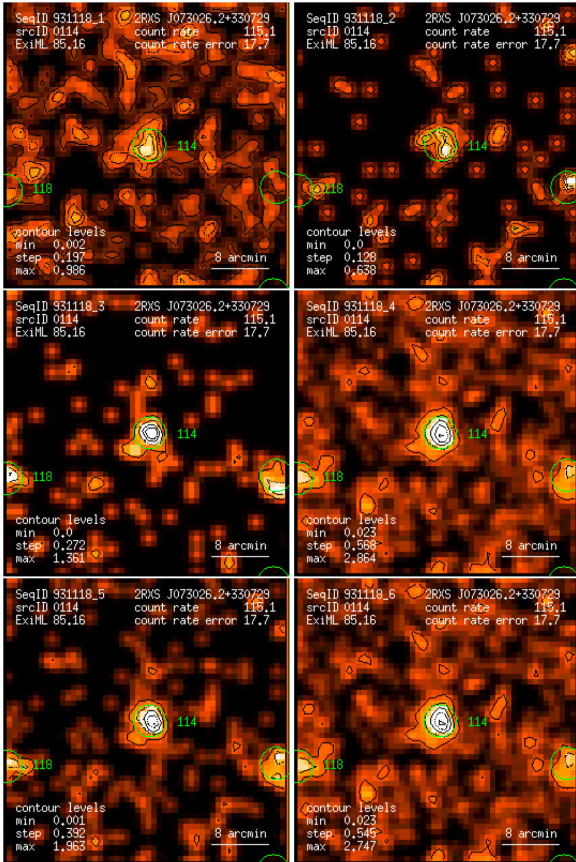
Figure 114: RASS 931118: detection 0114: band rate images, Gaussian filter: (1) PSPC channels 11 – 41, (2) 52 – 90, (3) 91 – 201, (4) 11 – 235, (5) 52 – 201, (6) 11 – 201. Broad band rates in counts/ks. Band rate contour levels in counts/ks/arcmin 2 .
