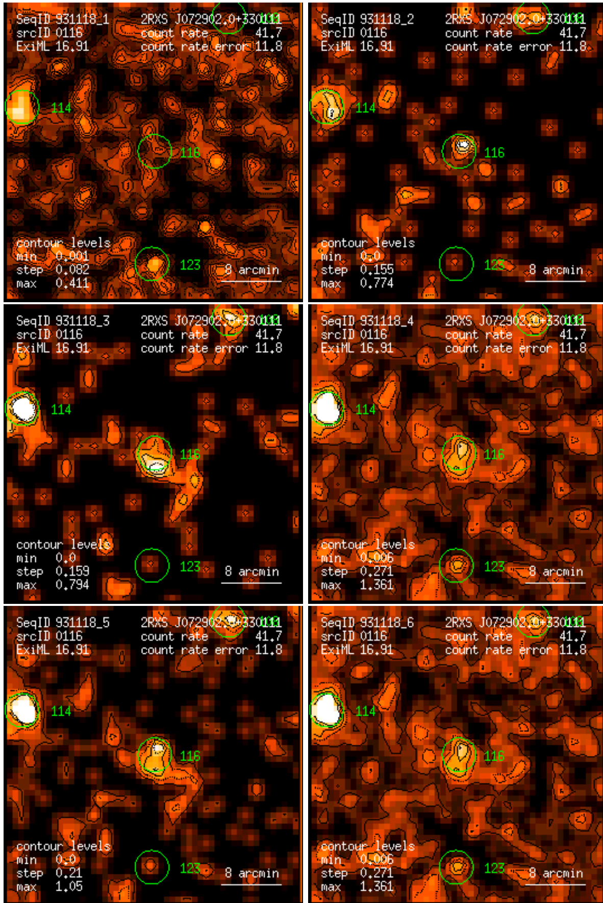
Figure 116: RASS 931118: detection 0116: band rate images, Gaussian filter: (1) PSPC channels 11 – 41, (2) 52 – 90, (3) 91 – 201, (4) 11 – 235, (5) 52 – 201, (6) 11 – 201. Broad band rates in counts/ks. Band rate contour levels in counts/ks/arcmin 2 .
