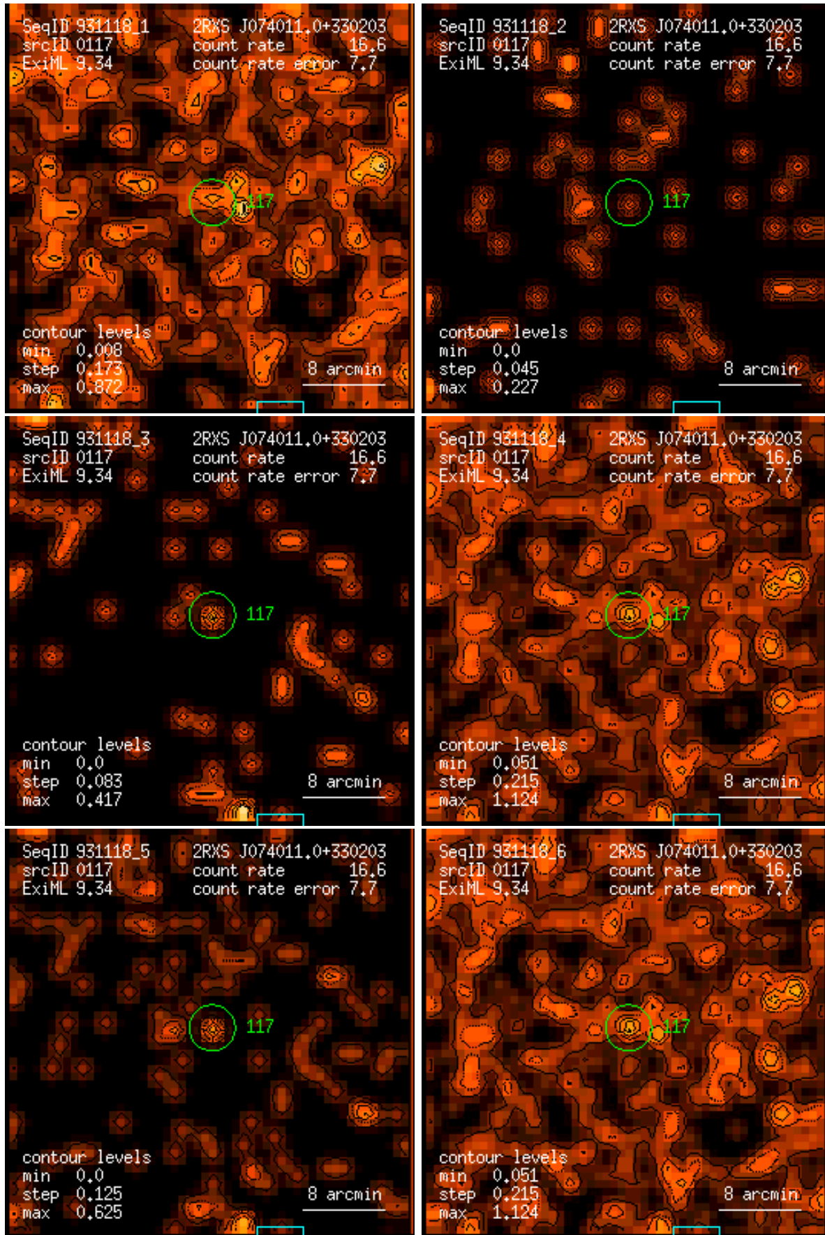
Figure 117: RASS 931118: detection 0117: band rate images, Gaussian filter: (1) PSPC channels 11 – 41, (2) 52 – 90, (3) 91 – 201, (4) 11 – 235, (5) 52 – 201, (6) 11 – 201. Broad band rates in counts/ks. Band rate contour levels in counts/ks/arcmin 2 .
