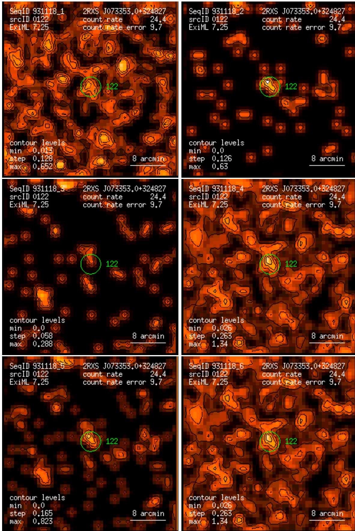
Figure 122: RASS 931118: detection 0122: band rate images, Gaussian filter: (1) PSPC channels 11 – 41, (2) 52 – 90, (3) 91 – 201, (4) 11 – 235, (5) 52 – 201, (6) 11 – 201. Broad band rates in counts/ks. Band rate contour levels in counts/ks/arcmin 2 .
