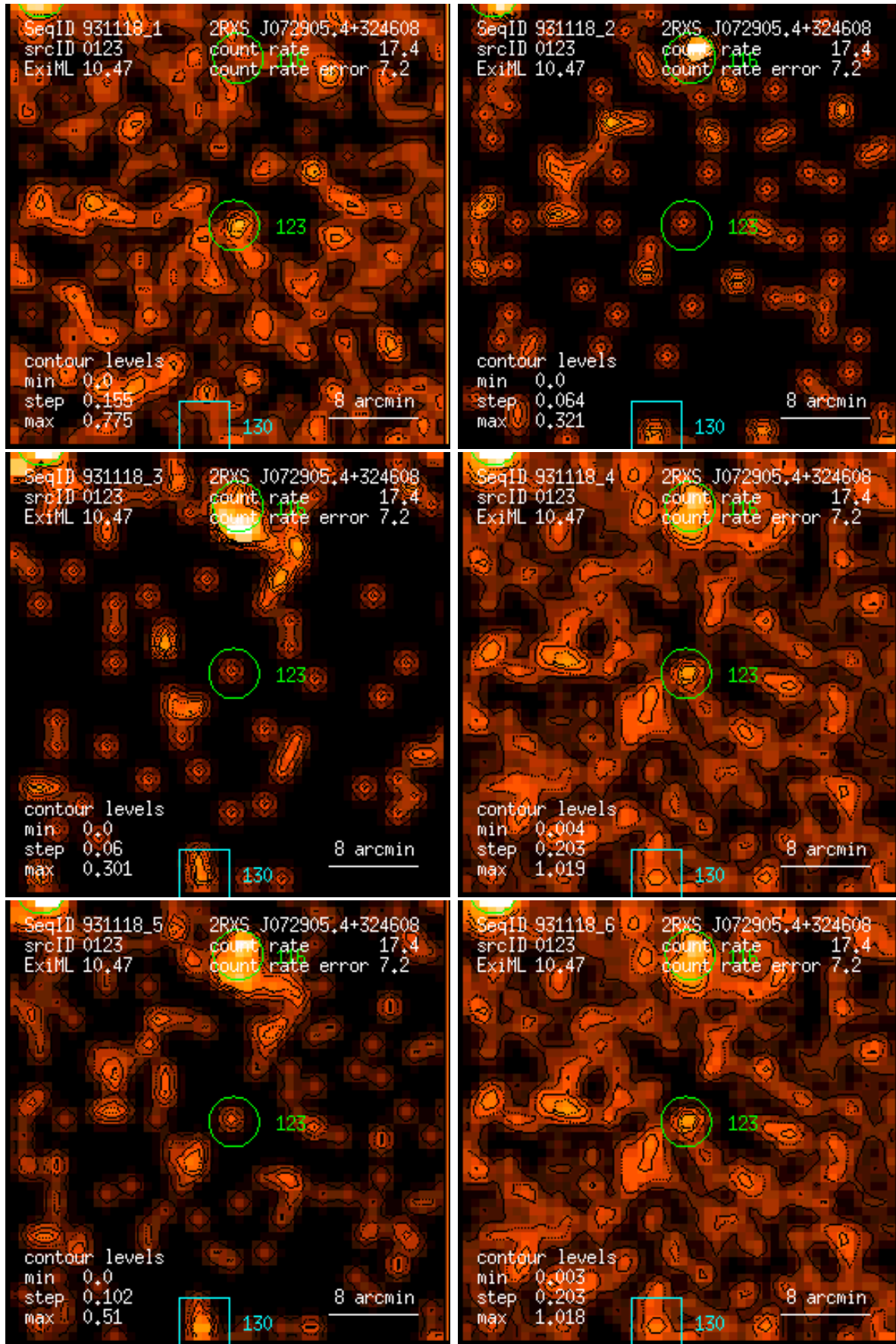
Figure 123: RASS 931118: detection 0123: band rate images, Gaussian filter: (1) PSPC channels 11 – 41, (2) 52 – 90, (3) 91 – 201, (4) 11 – 235, (5) 52 – 201, (6) 11 – 201. Broad band rates in counts/ks. Band rate contour levels in counts/ks/arcmin 2 .
