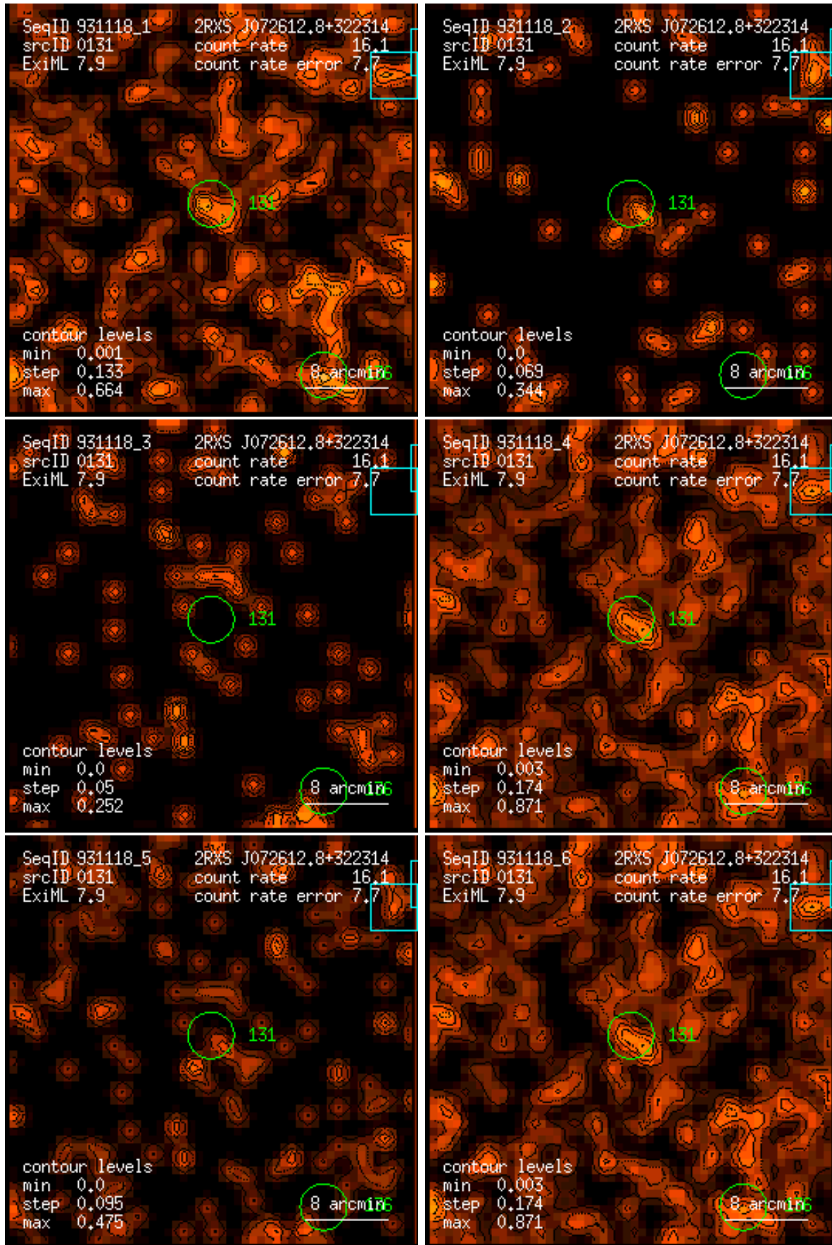
Figure 131: RASS 931118: detection 0131: band rate images, Gaussian filter: (1) PSPC channels 11 – 41, (2) 52 – 90, (3) 91 – 201, (4) 11 – 235, (5) 52 – 201, (6) 11 – 201. Broad band rates in counts/ks. Band rate contour levels in counts/ks/arcmin 2 .
