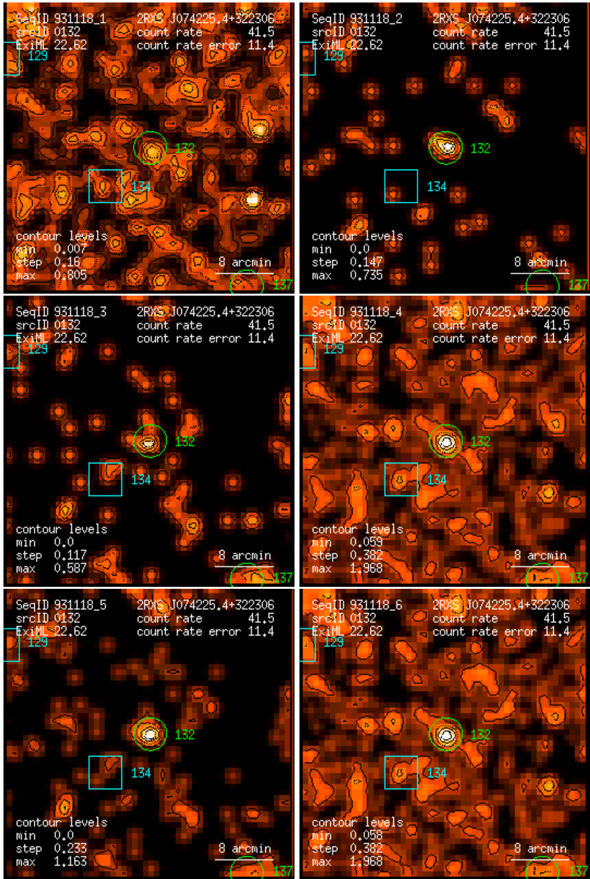
Figure 132: RASS 931118: detection 0132: band rate images, Gaussian filter: (1) PSPC channels 11 – 41, (2) 52 – 90, (3) 91 – 201, (4) 11 – 235, (5) 52 – 201, (6) 11 – 201. Broad band rates in counts/ks. Band rate contour levels in counts/ks/arcmin 2 .
