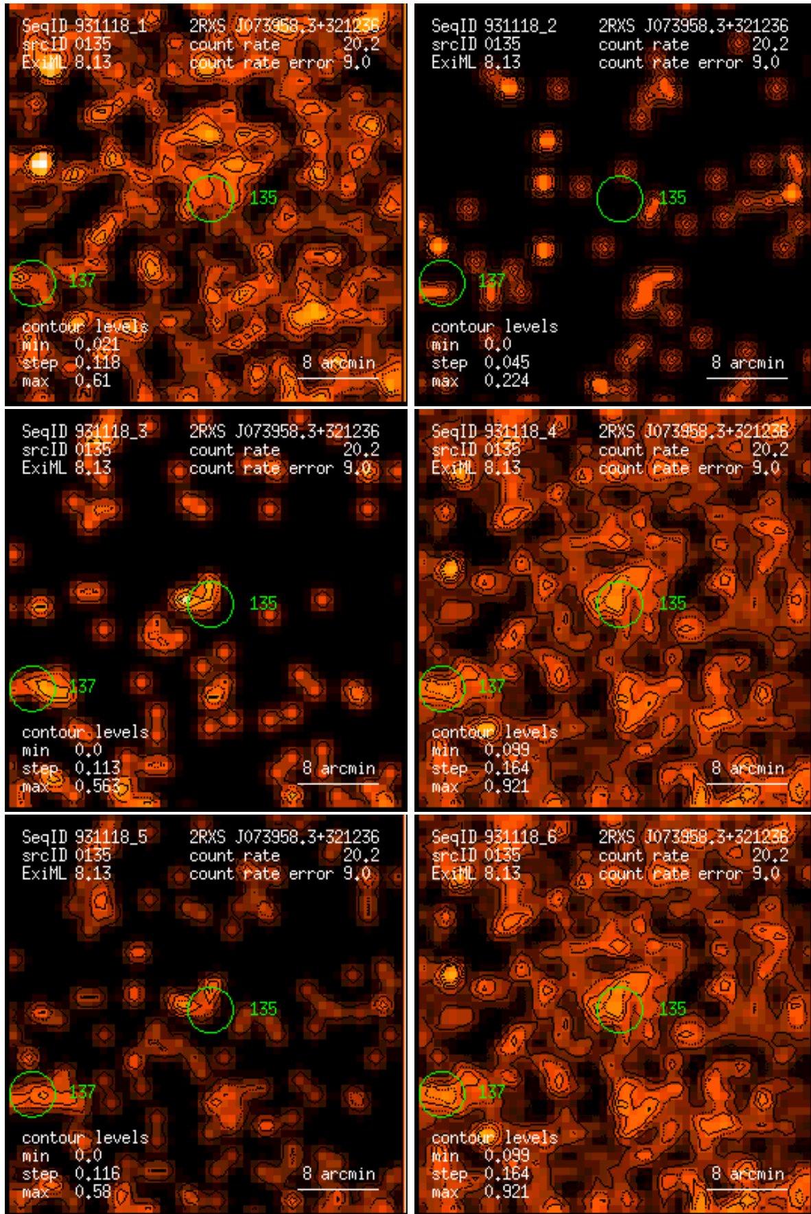
Figure 135: RASS 931118: detection 0135: band rate images, Gaussian filter: (1) PSPC channels 11 – 41, (2) 52 – 90, (3) 91 – 201, (4) 11 – 235, (5) 52 – 201, (6) 11 – 201. Broad band rates in counts/ks. Band rate contour levels in counts/ks/arcmin 2 .
