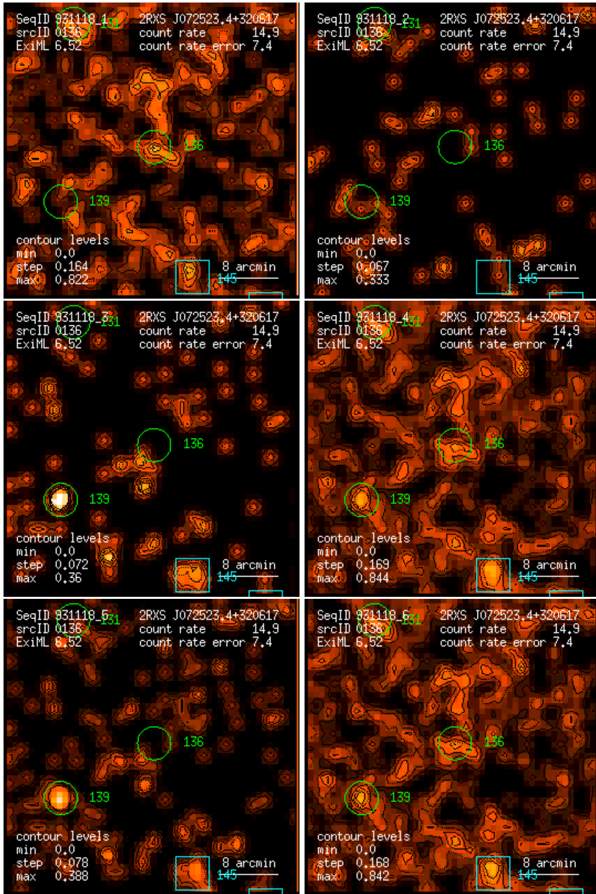
Figure 136: RASS 931118: detection 0136: band rate images, Gaussian filter: (1) PSPC channels 11 – 41, (2) 52 – 90, (3) 91 – 201, (4) 11 – 235, (5) 52 – 201, (6) 11 – 201. Broad band rates in counts/ks. Band rate contour levels in counts/ks/arcmin 2 .
