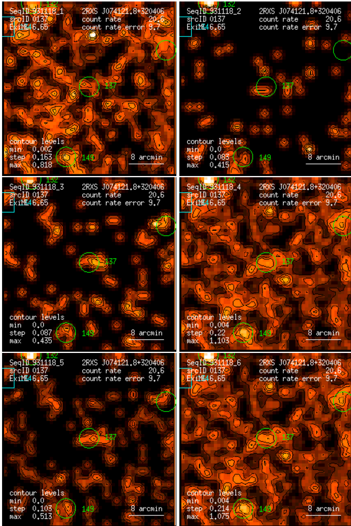
Figure 137: RASS 931118: detection 0137: band rate images, Gaussian filter: (1) PSPC channels 11 – 41, (2) 52 – 90, (3) 91 – 201, (4) 11 – 235, (5) 52 – 201, (6) 11 – 201. Broad band rates in counts/ks. Band rate contour levels in counts/ks/arcmin 2 .
