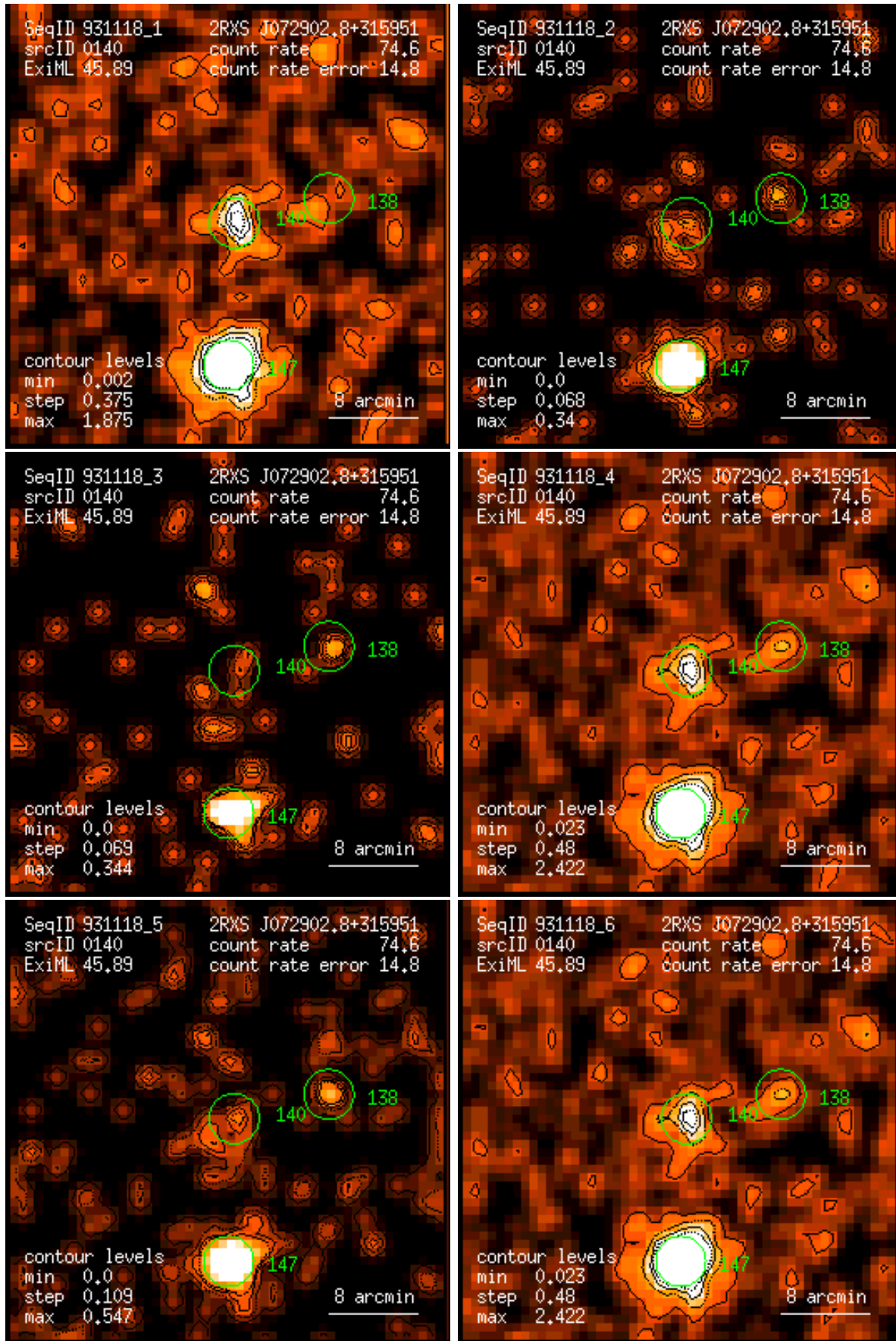
Figure 140: RASS 931118: detection 0140: band rate images, Gaussian filter: (1) PSPC channels 11 – 41, (2) 52 – 90, (3) 91 – 201, (4) 11 – 235, (5) 52 – 201, (6) 11 – 201. Broad band rates in counts/ks. Band rate contour levels in counts/ks/arcmin 2 .
