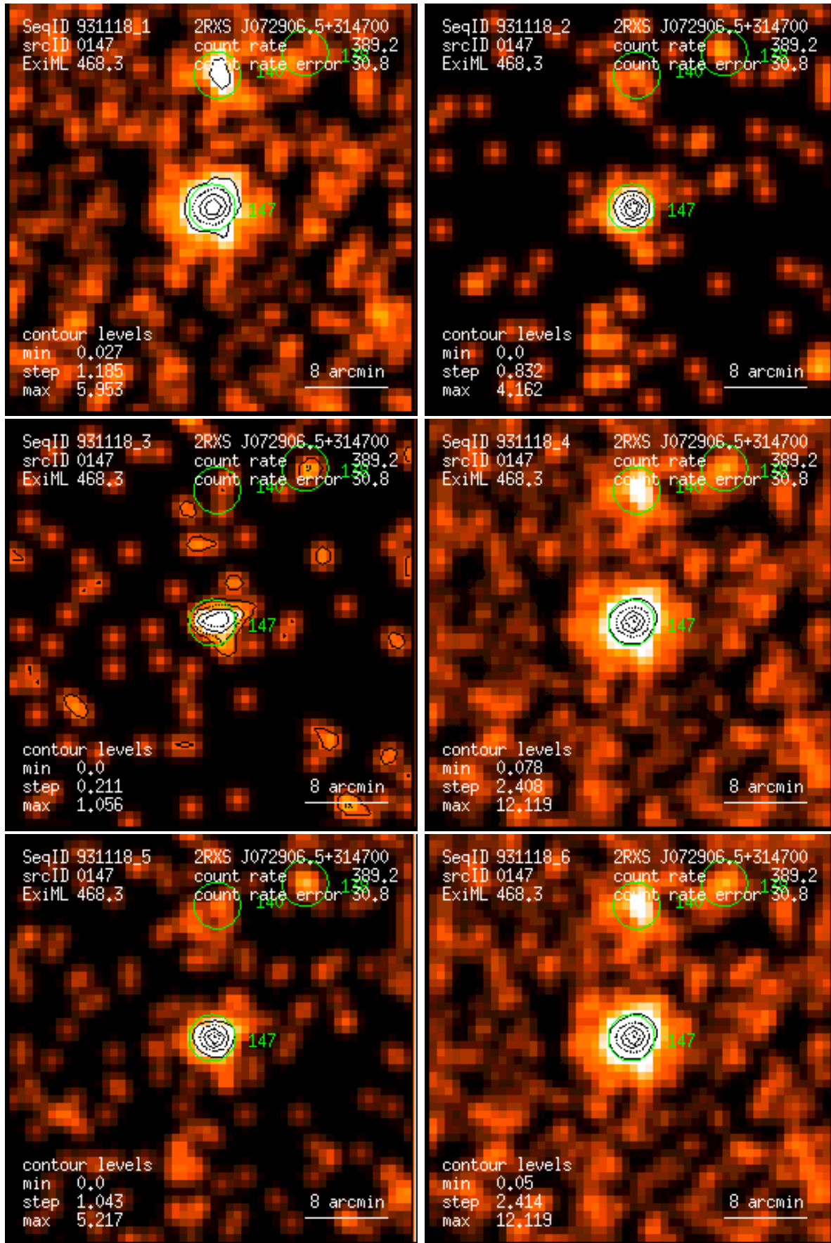
Figure 147: RASS 931118: detection 0147: band rate images, Gaussian filter: (1) PSPC channels 11 – 41, (2) 52 – 90, (3) 91 – 201, (4) 11 – 235, (5) 52 – 201, (6) 11 – 201. Broad band rates in counts/ks. Band rate contour levels in counts/ks/arcmin 2 .
