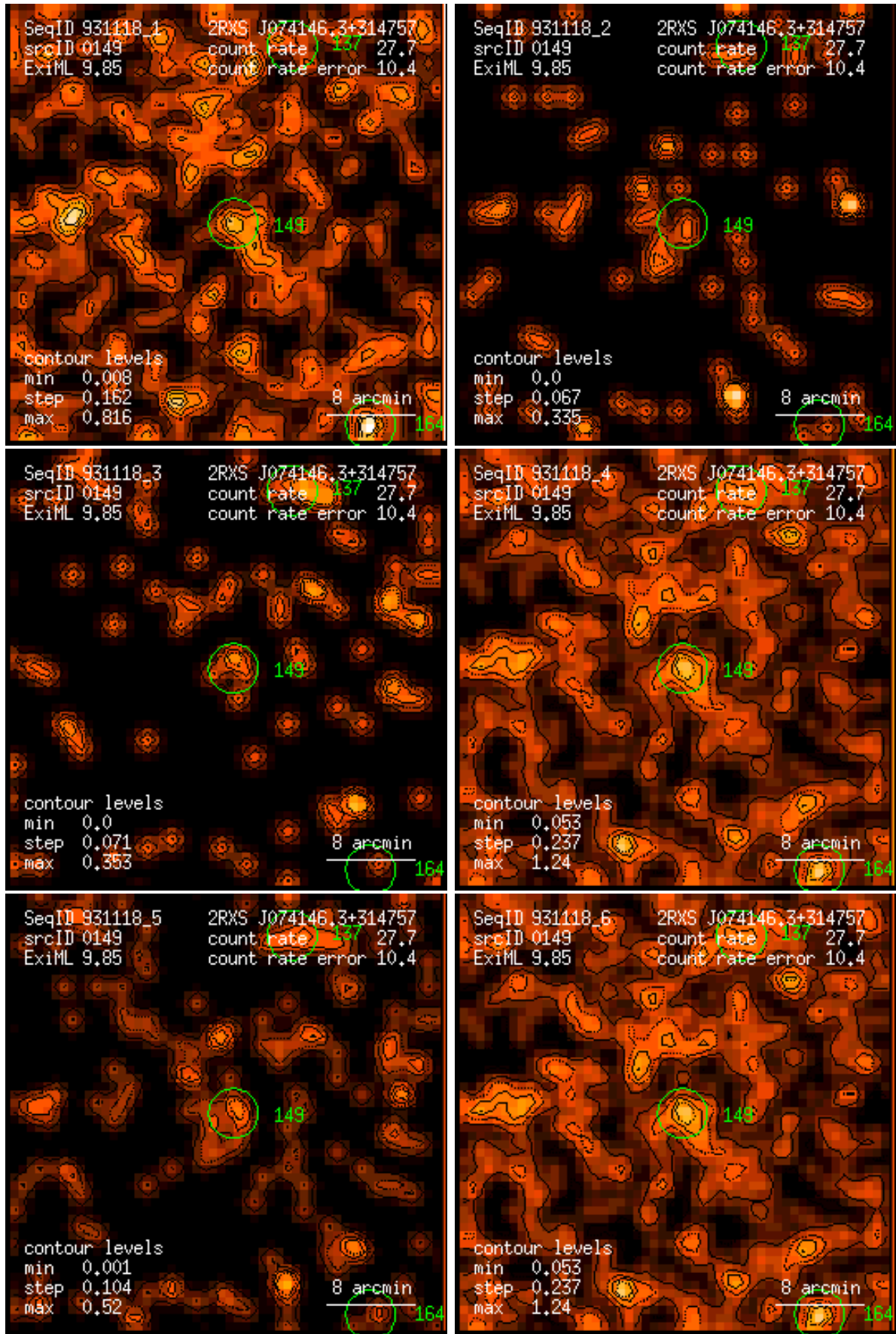
Figure 149: RASS 931118: detection 0149: band rate images, Gaussian filter: (1) PSPC channels 11 – 41, (2) 52 – 90, (3) 91 – 201, (4) 11 – 235, (5) 52 – 201, (6) 11 – 201. Broad band rates in counts/ks. Band rate contour levels in counts/ks/arcmin 2 .
