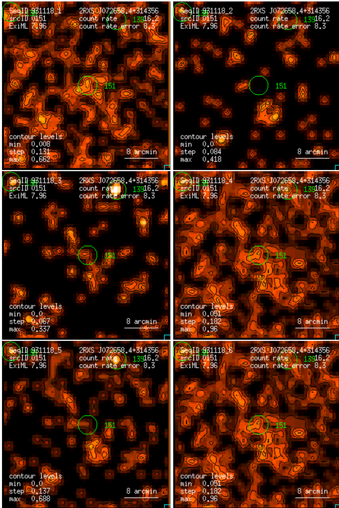
Figure 151: RASS 931118: detection 0151: band rate images, Gaussian filter: (1) PSPC channels 11 – 41, (2) 52 – 90, (3) 91 – 201, (4) 11 – 235, (5) 52 – 201, (6) 11 – 201. Broad band rates in counts/ks. Band rate contour levels in counts/ks/arcmin 2 .
