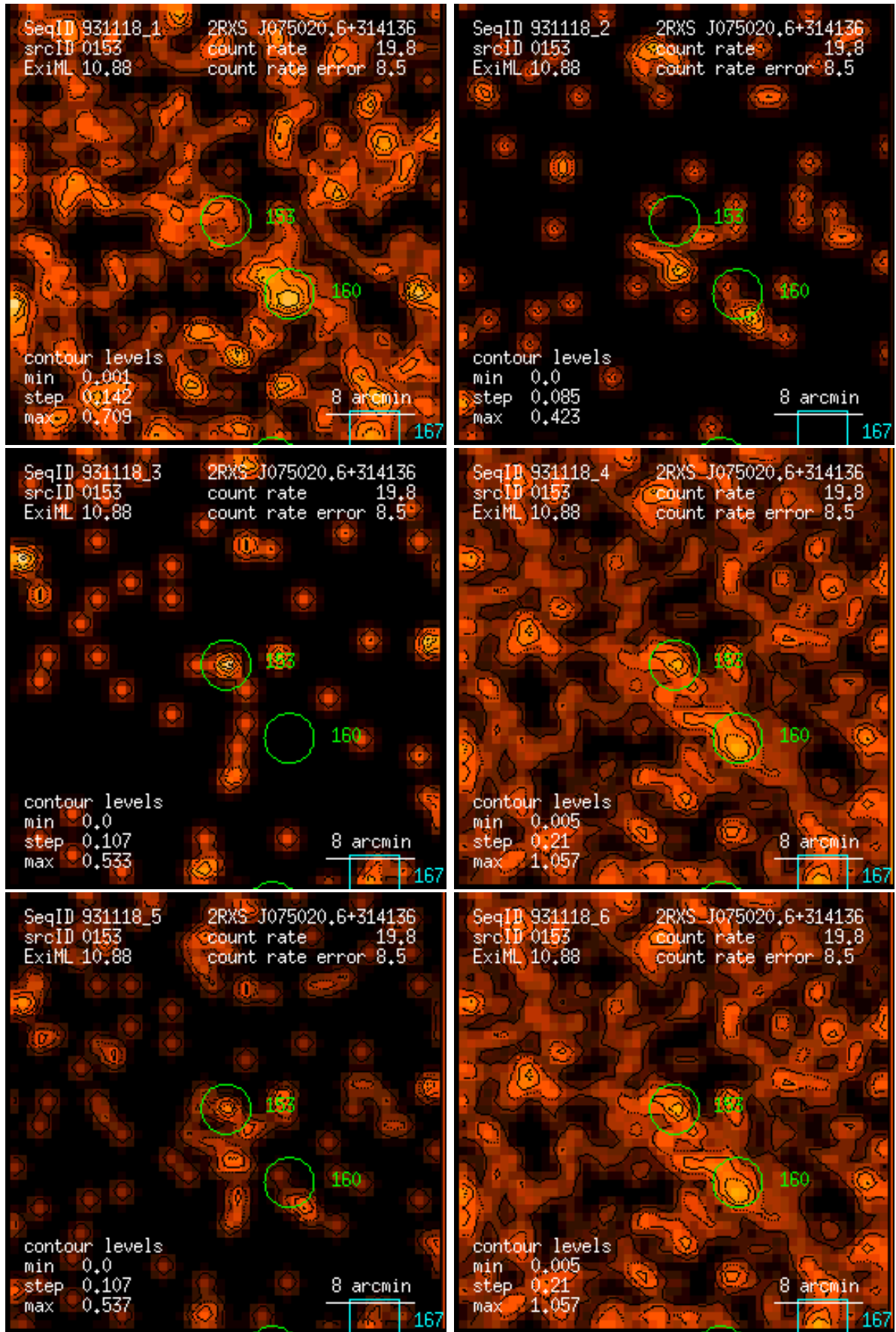
Figure 153: RASS 931118: detection 0153: band rate images, Gaussian filter: (1) PSPC channels 11 – 41, (2) 52 – 90, (3) 91 – 201, (4) 11 – 235, (5) 52 – 201, (6) 11 – 201. Broad band rates in counts/ks. Band rate contour levels in counts/ks/arcmin 2 .
