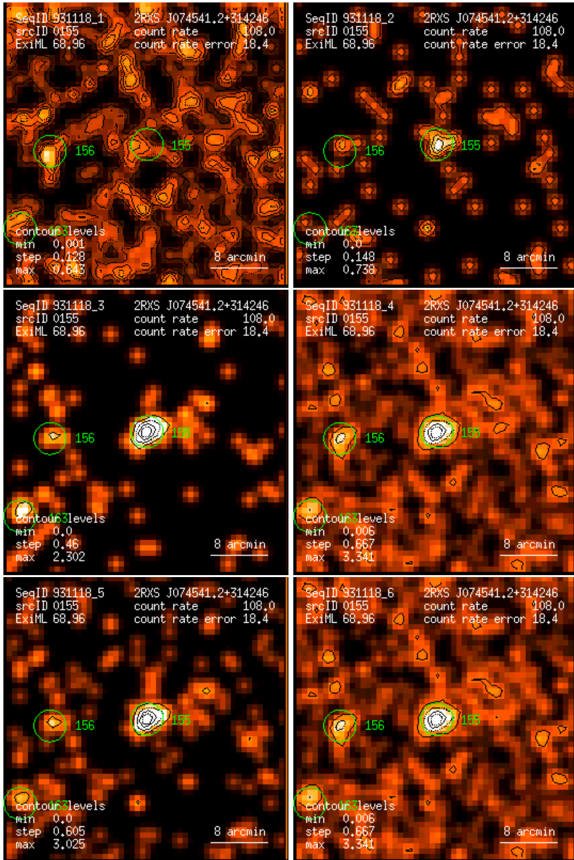
Figure 155: RASS 931118: detection 0155: band rate images, Gaussian filter: (1) PSPC channels 11 – 41, (2) 52 – 90, (3) 91 – 201, (4) 11 – 235, (5) 52 – 201, (6) 11 – 201. Broad band rates in counts/ks. Band rate contour levels in counts/ks/arcmin 2 .
