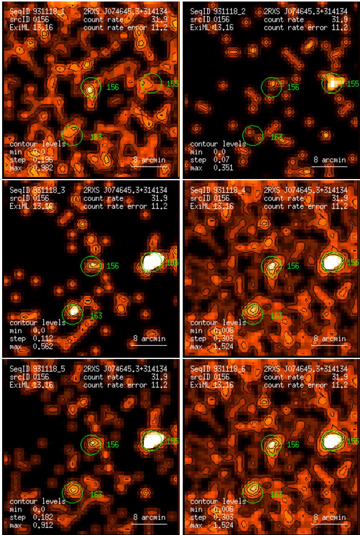
Figure 156: RASS 931118: detection 0156: band rate images, Gaussian filter: (1) PSPC channels 11 – 41, (2) 52 – 90, (3) 91 – 201, (4) 11 – 235, (5) 52 – 201, (6) 11 – 201. Broad band rates in counts/ks. Band rate contour levels in counts/ks/arcmin 2 .
