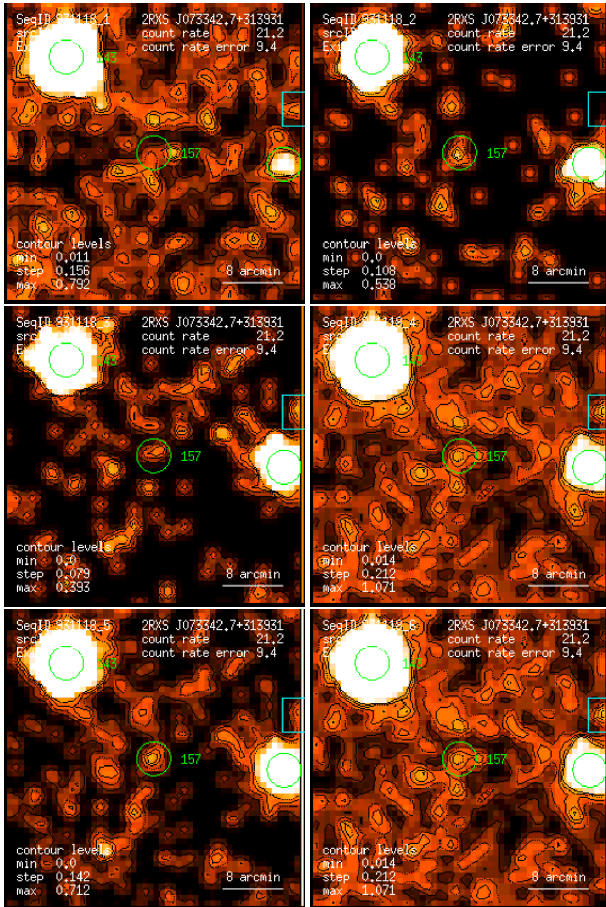
Figure 157: RASS 931118: detection 0157: band rate images, Gaussian filter: (1) PSPC channels 11 – 41, (2) 52 – 90, (3) 91 – 201, (4) 11 – 235, (5) 52 – 201, (6) 11 – 201. Broad band rates in counts/ks. Band rate contour levels in counts/ks/arcmin 2 .
