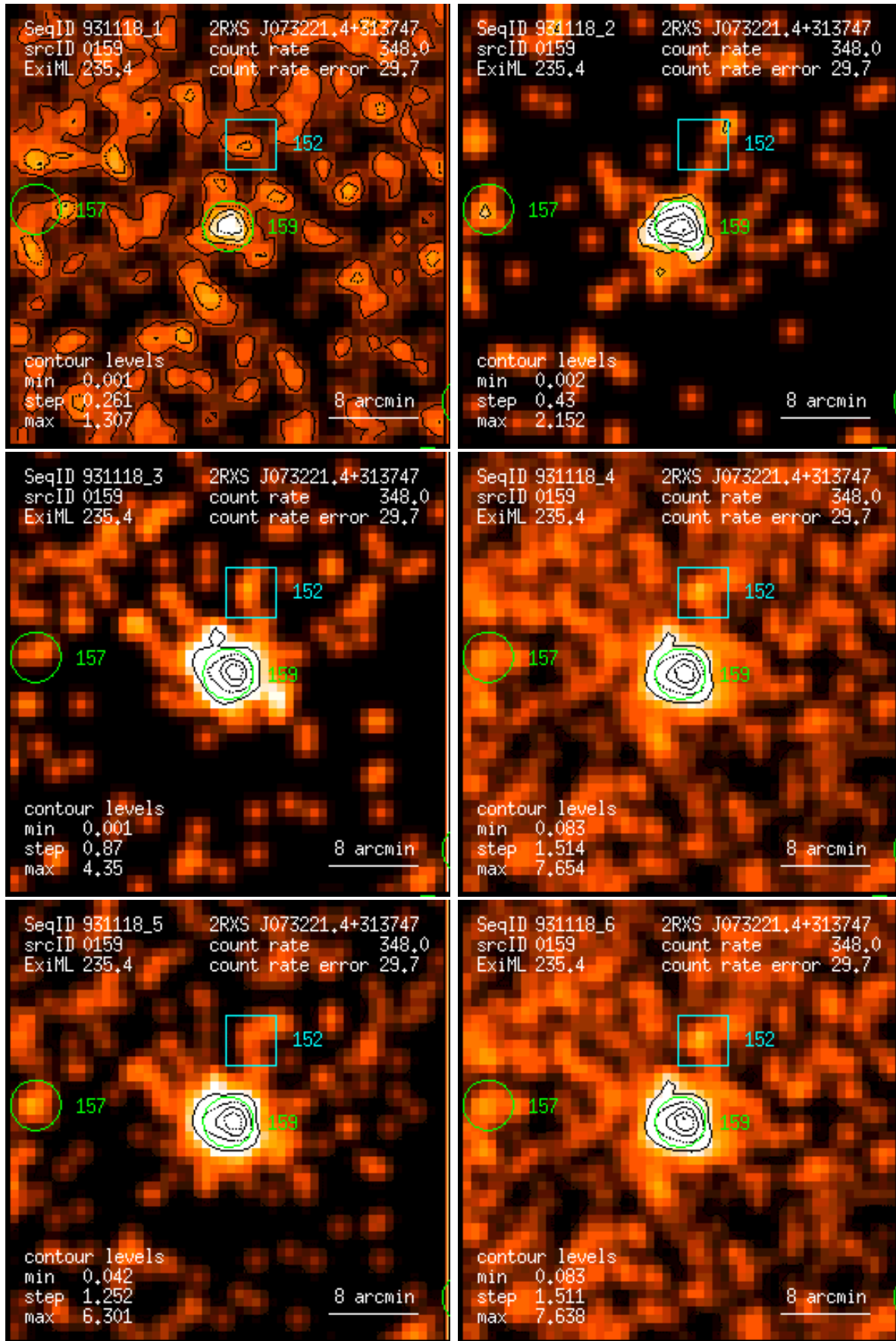
Figure 159: RASS 931118: detection 0159: band rate images, Gaussian filter: (1) PSPC channels 11 – 41, (2) 52 – 90, (3) 91 – 201, (4) 11 – 235, (5) 52 – 201, (6) 11 – 201. Broad band rates in counts/ks. Band rate contour levels in counts/ks/arcmin 2 .
