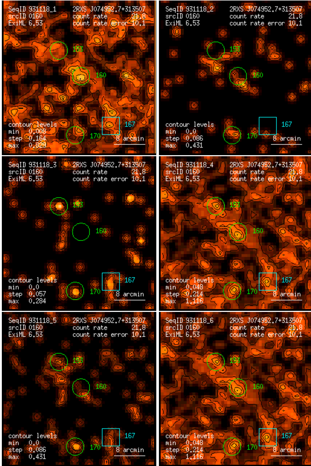
Figure 160: RASS 931118: detection 0160: band rate images, Gaussian filter: (1) PSPC channels 11 – 41, (2) 52 – 90, (3) 91 – 201, (4) 11 – 235, (5) 52 – 201, (6) 11 – 201. Broad band rates in counts/ks. Band rate contour levels in counts/ks/arcmin 2 .
