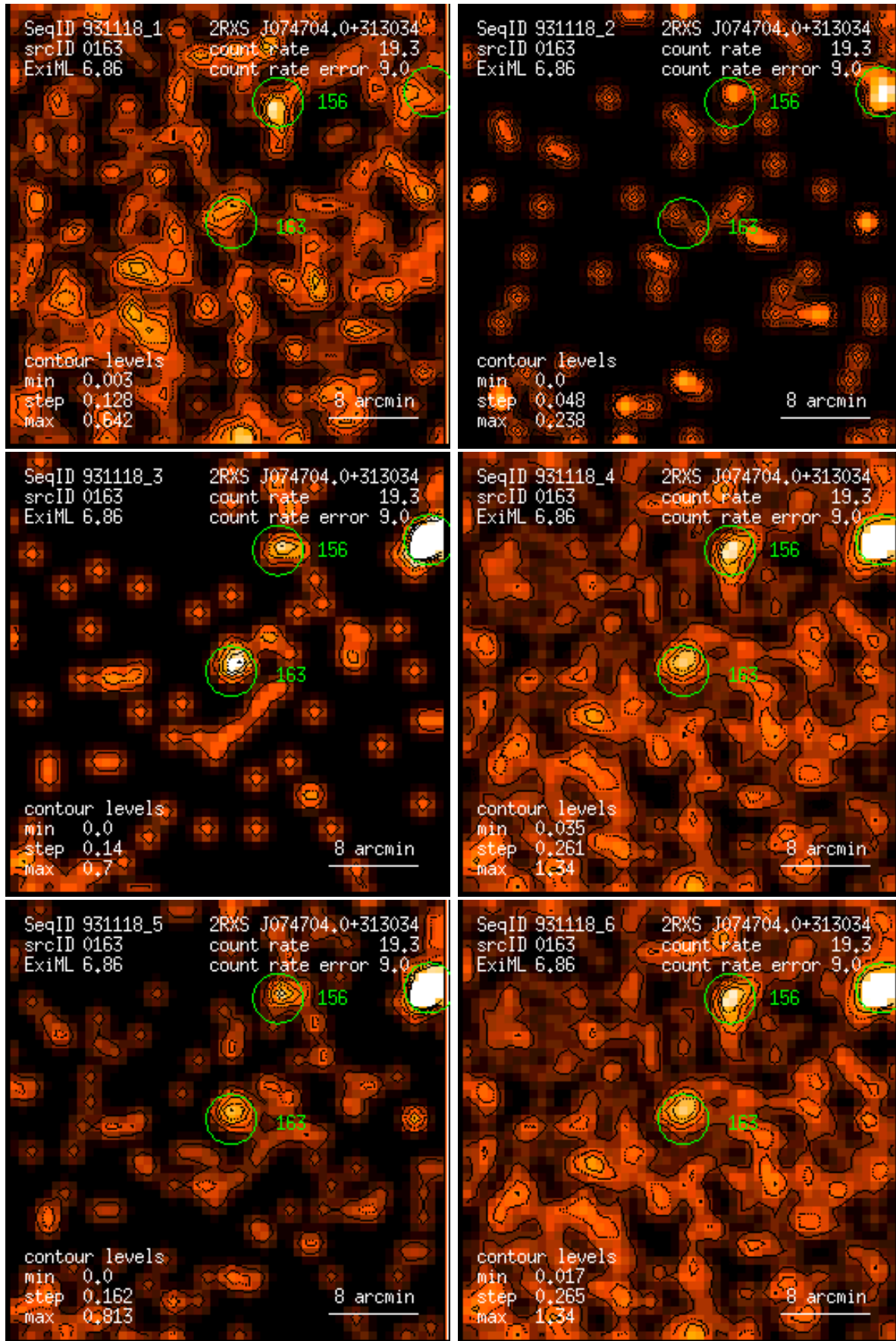
Figure 163: RASS 931118: detection 0163: band rate images, Gaussian filter: (1) PSPC channels 11 – 41, (2) 52 – 90, (3) 91 – 201, (4) 11 – 235, (5) 52 – 201, (6) 11 – 201. Broad band rates in counts/ks. Band rate contour levels in counts/ks/arcmin 2 .
