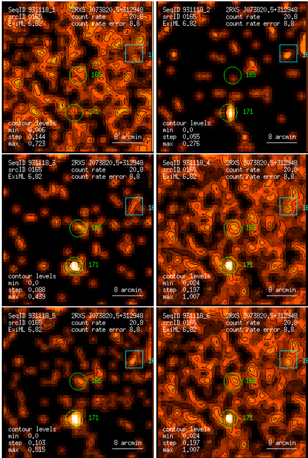
Figure 165: RASS 931118: detection 0165: band rate images, Gaussian filter: (1) PSPC channels 11 – 41, (2) 52 – 90, (3) 91 – 201, (4) 11 – 235, (5) 52 – 201, (6) 11 – 201. Broad band rates in counts/ks. Band rate contour levels in counts/ks/arcmin 2 .
