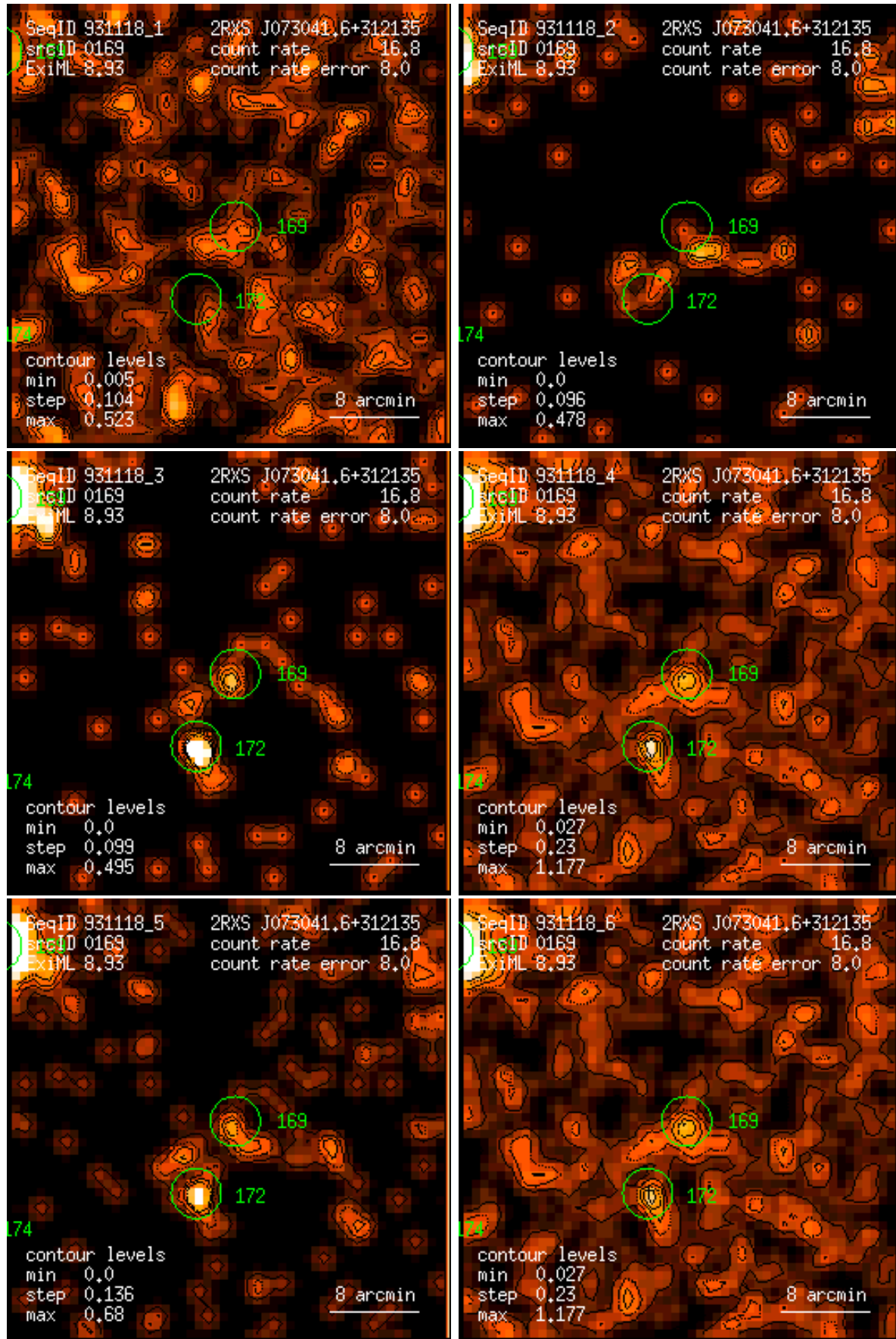
Figure 169: RASS 931118: detection 0169: band rate images, Gaussian filter: (1) PSPC channels 11 – 41, (2) 52 – 90, (3) 91 – 201, (4) 11 – 235, (5) 52 – 201, (6) 11 – 201. Broad band rates in counts/ks. Band rate contour levels in counts/ks/arcmin 2 .
