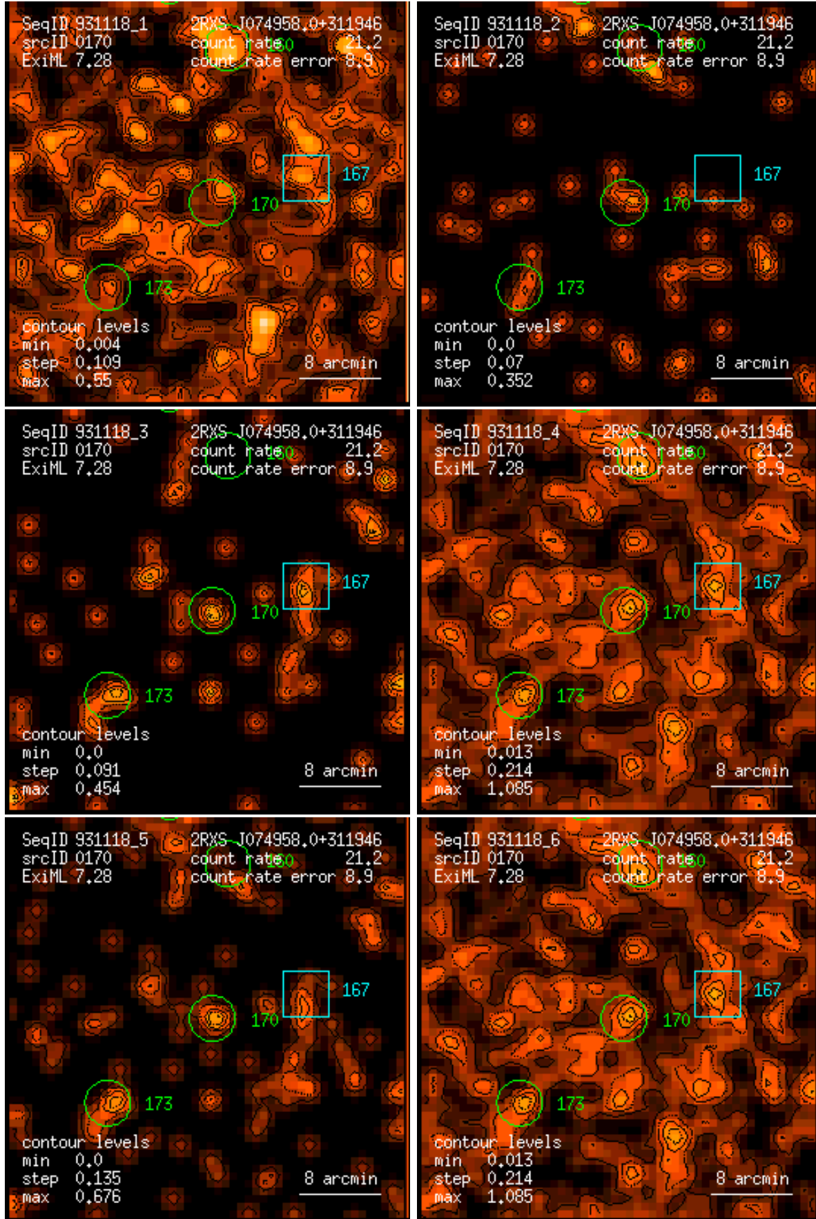
Figure 170: RASS 931118: detection 0170: band rate images, Gaussian filter: (1) PSPC channels 11 – 41, (2) 52 – 90, (3) 91 – 201, (4) 11 – 235, (5) 52 – 201, (6) 11 – 201. Broad band rates in counts/ks. Band rate contour levels in counts/ks/arcmin 2 .
