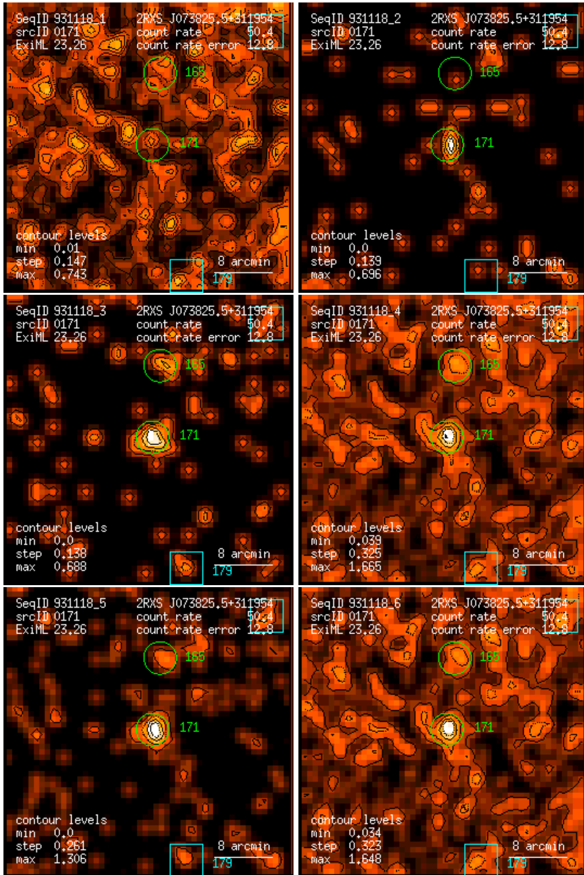
Figure 171: RASS 931118: detection 0171: band rate images, Gaussian filter: (1) PSPC channels 11 – 41, (2) 52 – 90, (3) 91 – 201, (4) 11 – 235, (5) 52 – 201, (6) 11 – 201. Broad band rates in counts/ks. Band rate contour levels in counts/ks/arcmin 2 .
