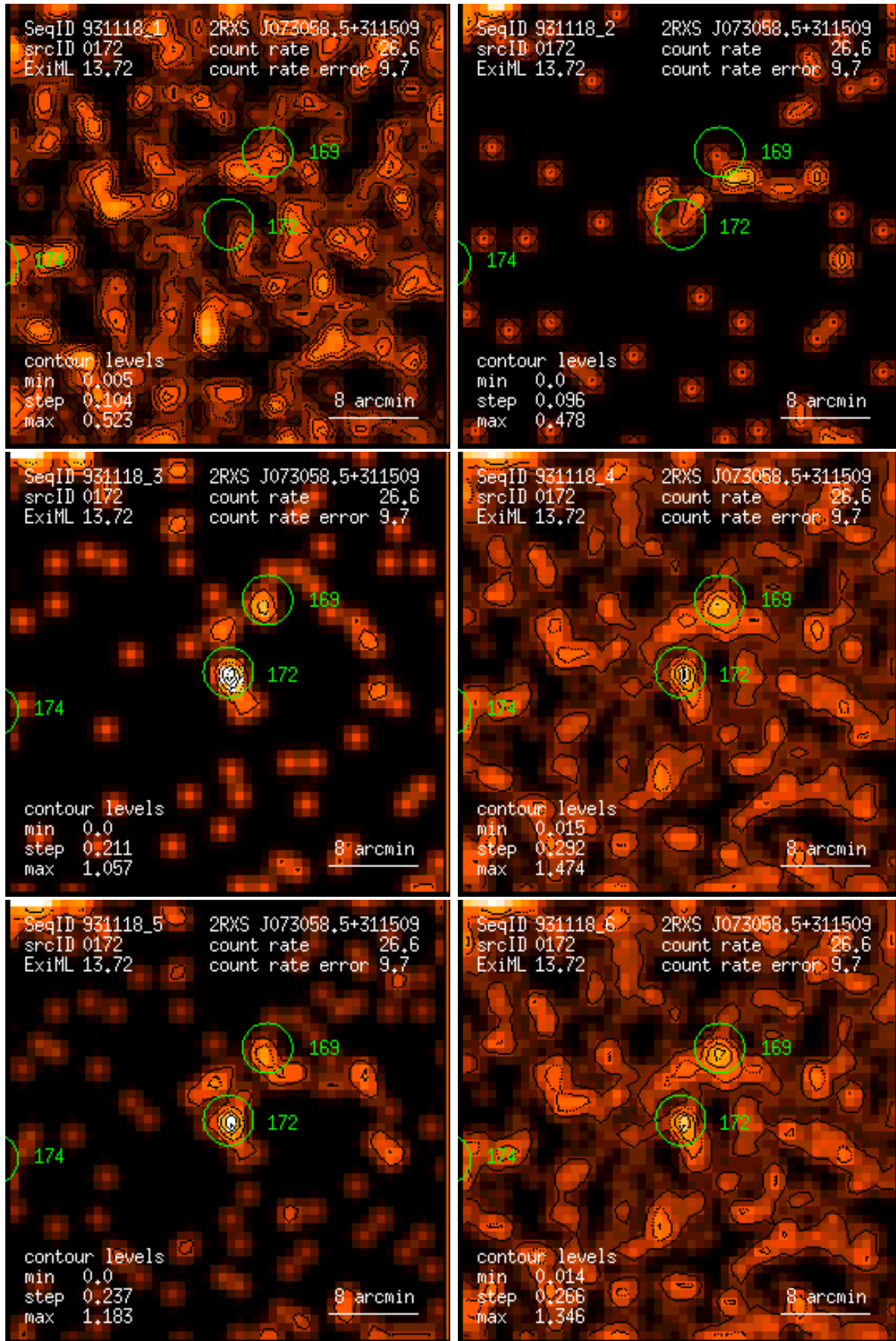
Figure 172: RASS 931118: detection 0172: band rate images, Gaussian filter: (1) PSPC channels 11 – 41, (2) 52 – 90, (3) 91 – 201, (4) 11 – 235, (5) 52 – 201, (6) 11 – 201. Broad band rates in counts/ks. Band rate contour levels in counts/ks/arcmin 2 .
