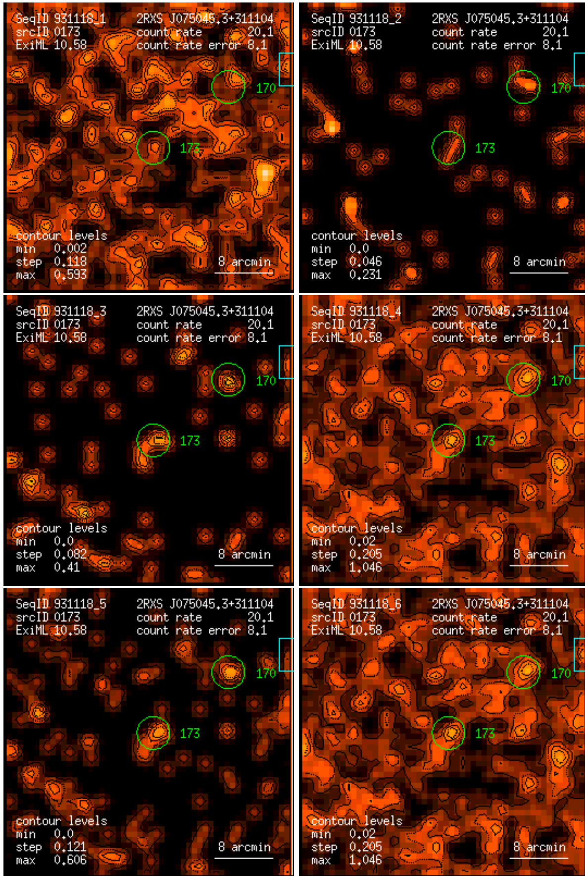
Figure 173: RASS 931118: detection 0173: band rate images, Gaussian filter: (1) PSPC channels 11 – 41, (2) 52 – 90, (3) 91 – 201, (4) 11 – 235, (5) 52 – 201, (6) 11 – 201. Broad band rates in counts/ks. Band rate contour levels in counts/ks/arcmin 2 .
