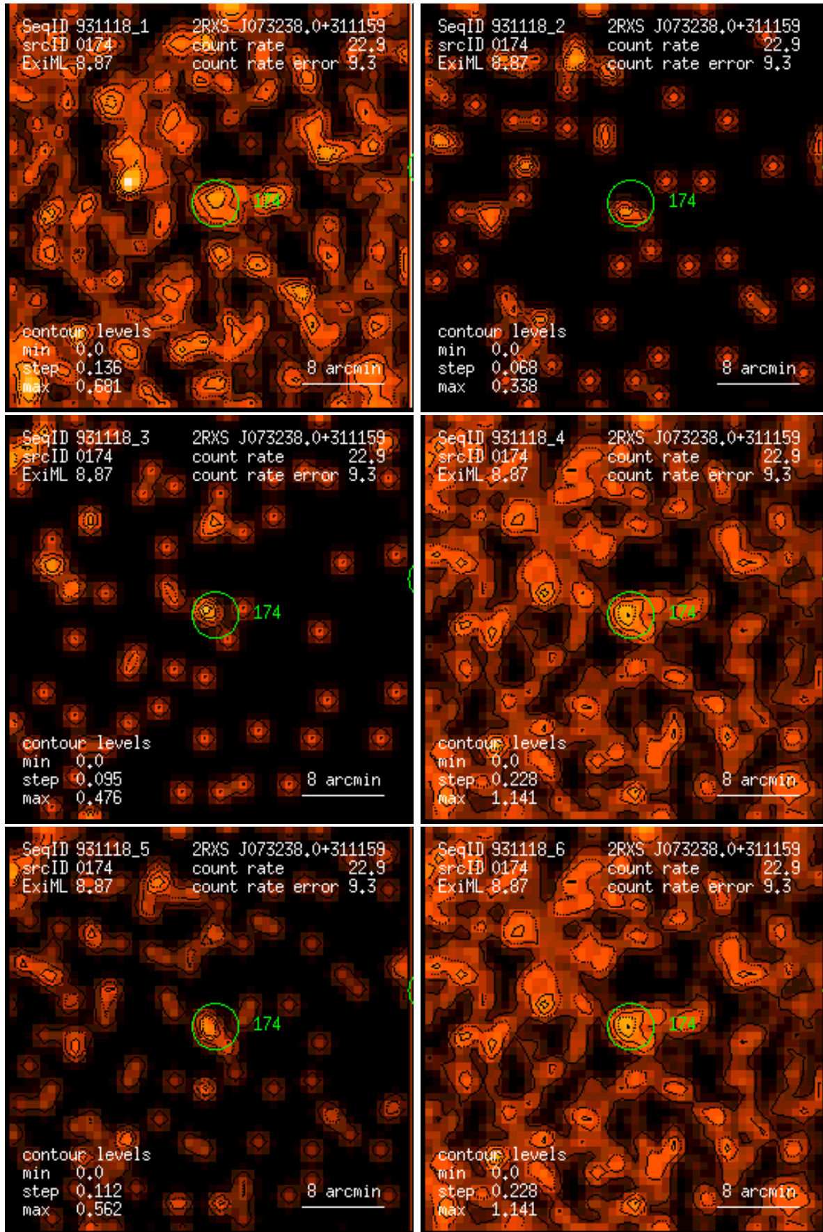
Figure 174: RASS 931118: detection 0174: band rate images, Gaussian filter: (1) PSPC channels 11 – 41, (2) 52 – 90, (3) 91 – 201, (4) 11 – 235, (5) 52 – 201, (6) 11 – 201. Broad band rates in counts/ks. Band rate contour levels in counts/ks/arcmin 2 .
