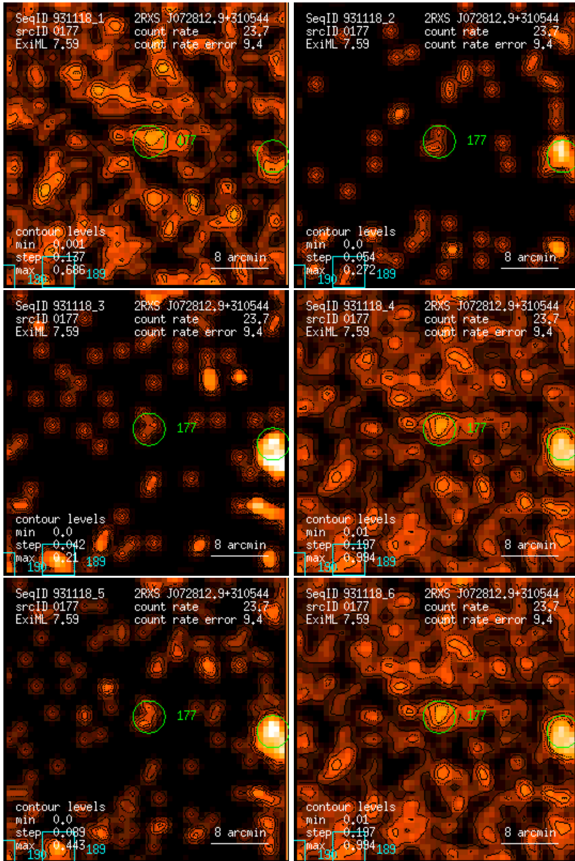
Figure 177: RASS 931118: detection 0177: band rate images, Gaussian filter: (1) PSPC channels 11 – 41, (2) 52 – 90, (3) 91 – 201, (4) 11 – 235, (5) 52 – 201, (6) 11 – 201. Broad band rates in counts/ks. Band rate contour levels in counts/ks/arcmin 2 .
