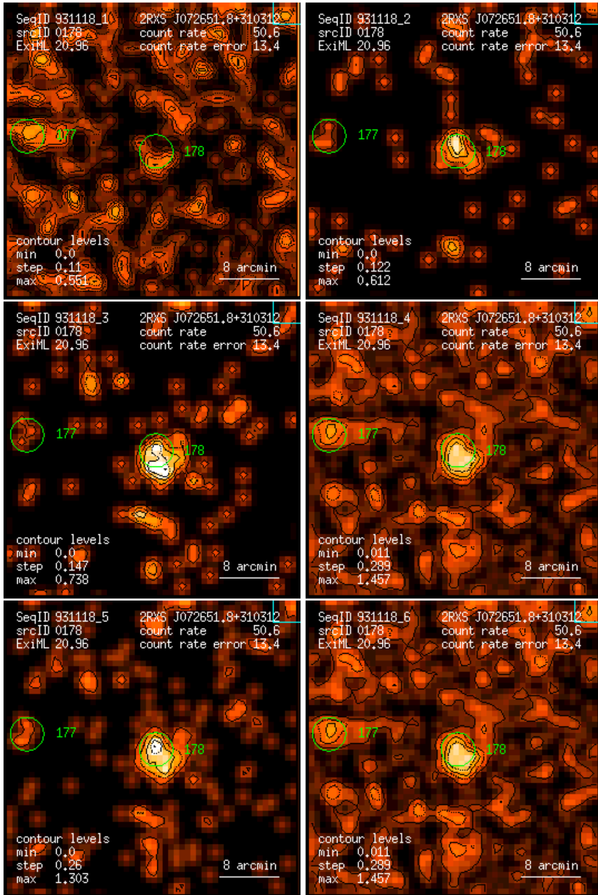
Figure 178: RASS 931118: detection 0178: band rate images, Gaussian filter: (1) PSPC channels 11 – 41, (2) 52 – 90, (3) 91 – 201, (4) 11 – 235, (5) 52 – 201, (6) 11 – 201. Broad band rates in counts/ks. Band rate contour levels in counts/ks/arcmin 2 .
