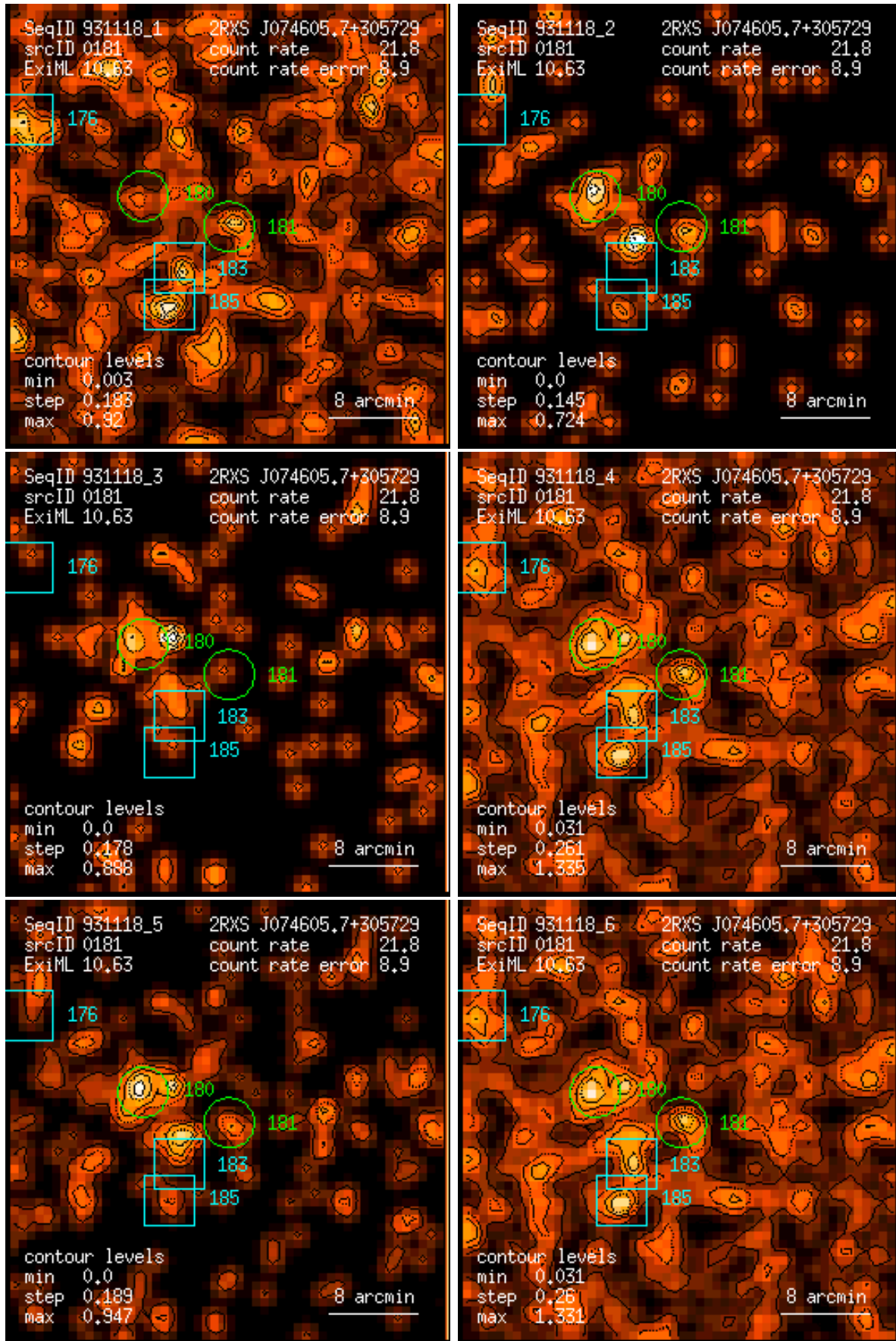
Figure 181: RASS 931118: detection 0181: band rate images, Gaussian filter: (1) PSPC channels 11 – 41, (2) 52 – 90, (3) 91 – 201, (4) 11 – 235, (5) 52 – 201, (6) 11 – 201. Broad band rates in counts/ks. Band rate contour levels in counts/ks/arcmin 2 .
