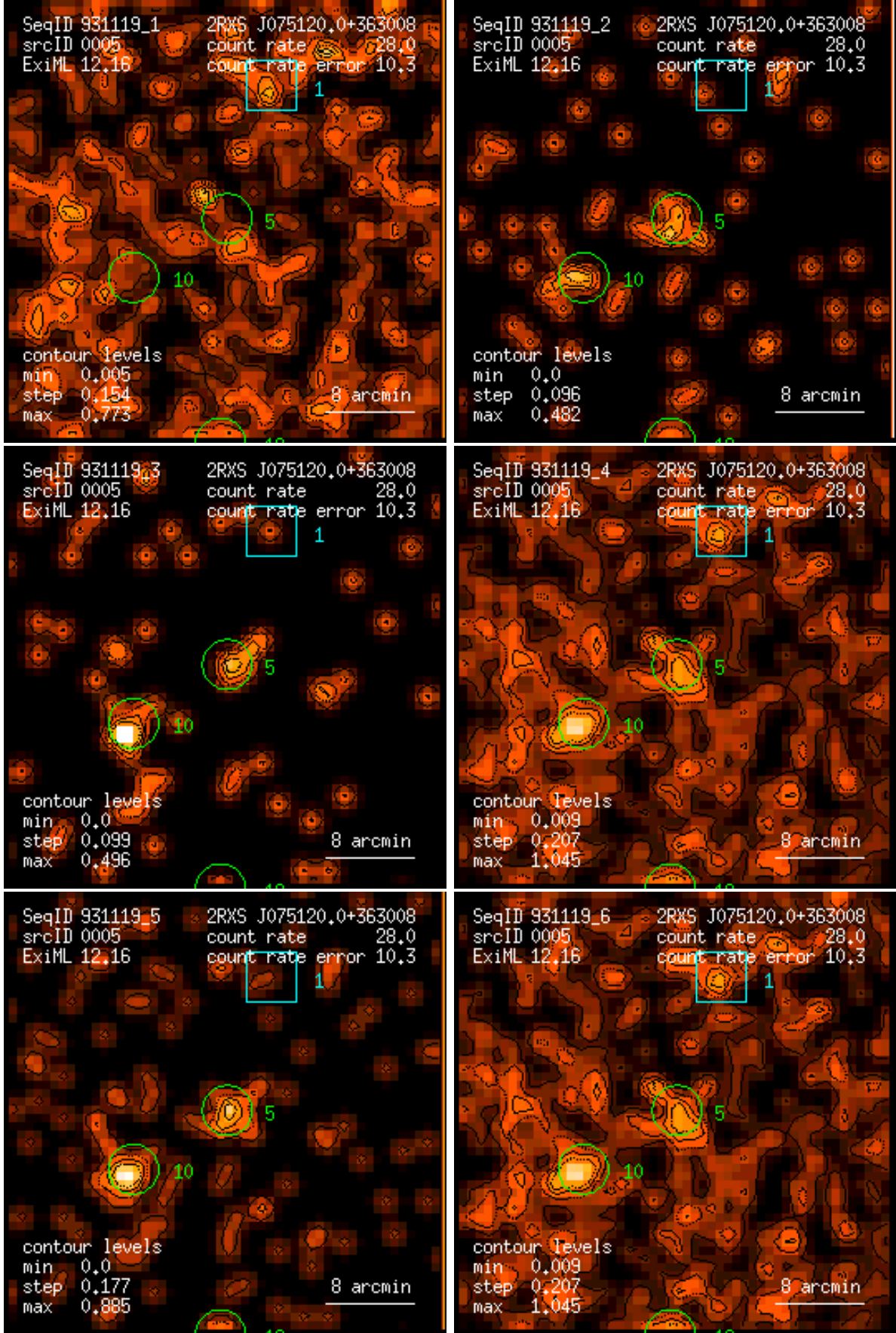
Figure 5: RASS 931119: detection 0005: band rate images, Gaussian filter: (1) PSPC channels 11 – 41, (2) 52 – 90, (3) 91 – 201, (4) 11 – 235, (5) 52 – 201, (6) 11 – 201. Broad band rates in counts/ks. Band rate contour levels in counts/ks/arcmin 2 .
