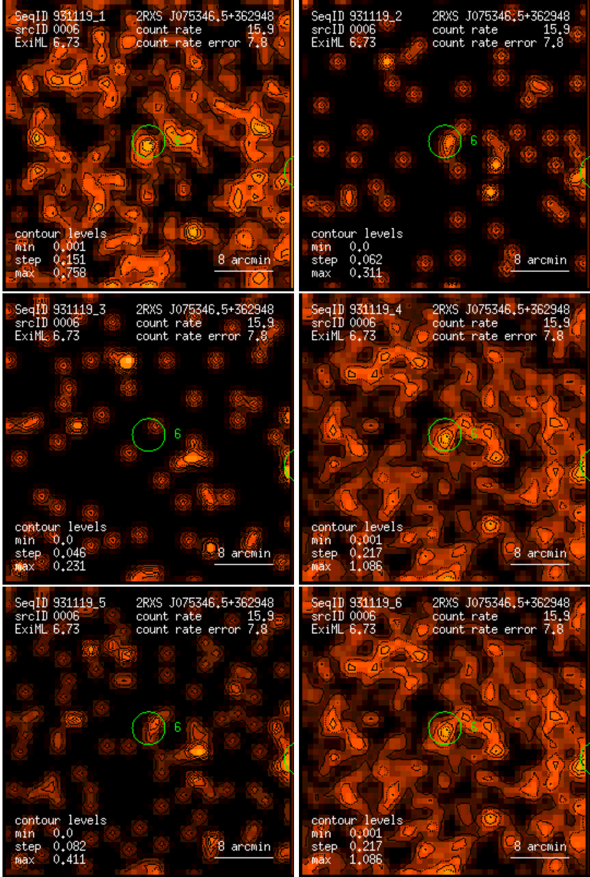
Figure 6: RASS 931119: detection 0006: band rate images, Gaussian filter: (1) PSPC channels 11 – 41, (2) 52 – 90, (3) 91 – 201, (4) 11 – 235, (5) 52 – 201, (6) 11 – 201. Broad band rates in counts/ks. Band rate contour levels in counts/ks/arcmin 2 .
