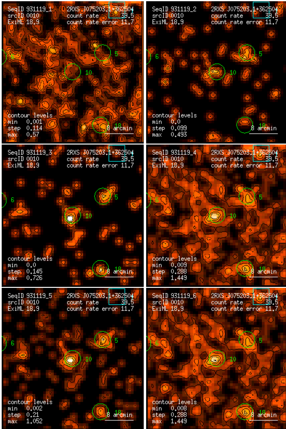
Figure 10: RASS 931119: detection 0010: band rate images, Gaussian filter: (1) PSPC channels 11 – 41, (2) 52 – 90, (3) 91 – 201, (4) 11 – 235, (5) 52 – 201, (6) 11 – 201. Broad band rates in counts/ks. Band rate contour levels in counts/ks/arcmin 2 .
