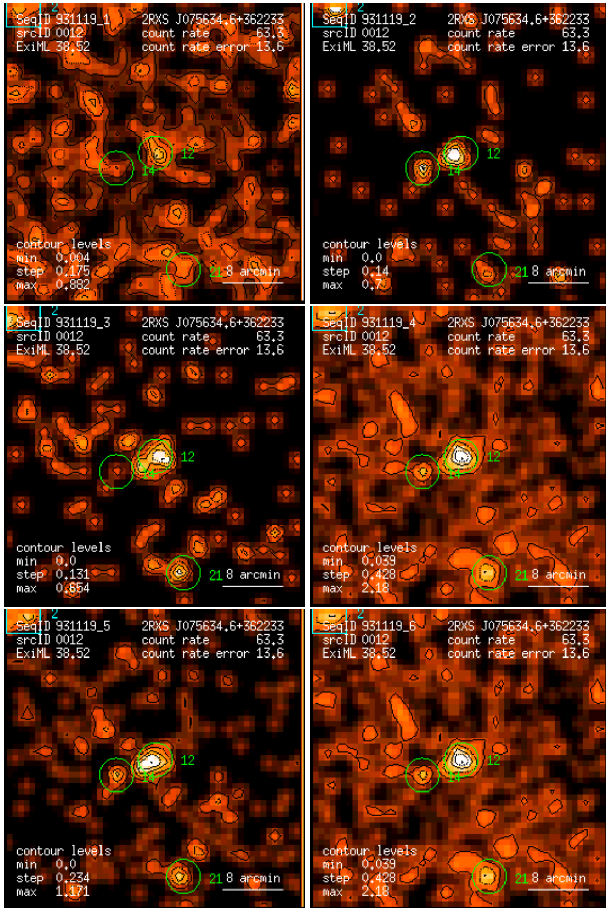
Figure 12: RASS 931119: detection 0012: band rate images, Gaussian filter: (1) PSPC channels 11 – 41, (2) 52 – 90, (3) 91 – 201, (4) 11 – 235, (5) 52 – 201, (6) 11 – 201. Broad band rates in counts/ks. Band rate contour levels in counts/ks/arcmin 2 .
